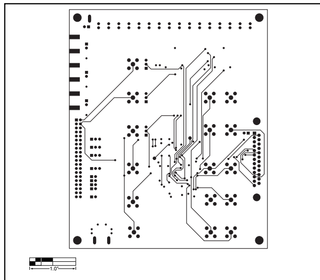
Figure 6. MXL1543 EV Kit PC Board Layout—Solder Side
