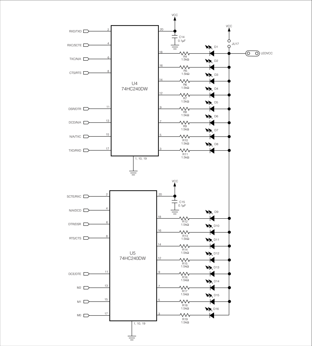
Figure 1b. MXL1543 EV Kit Schematic (Sheet 3 of 3)
