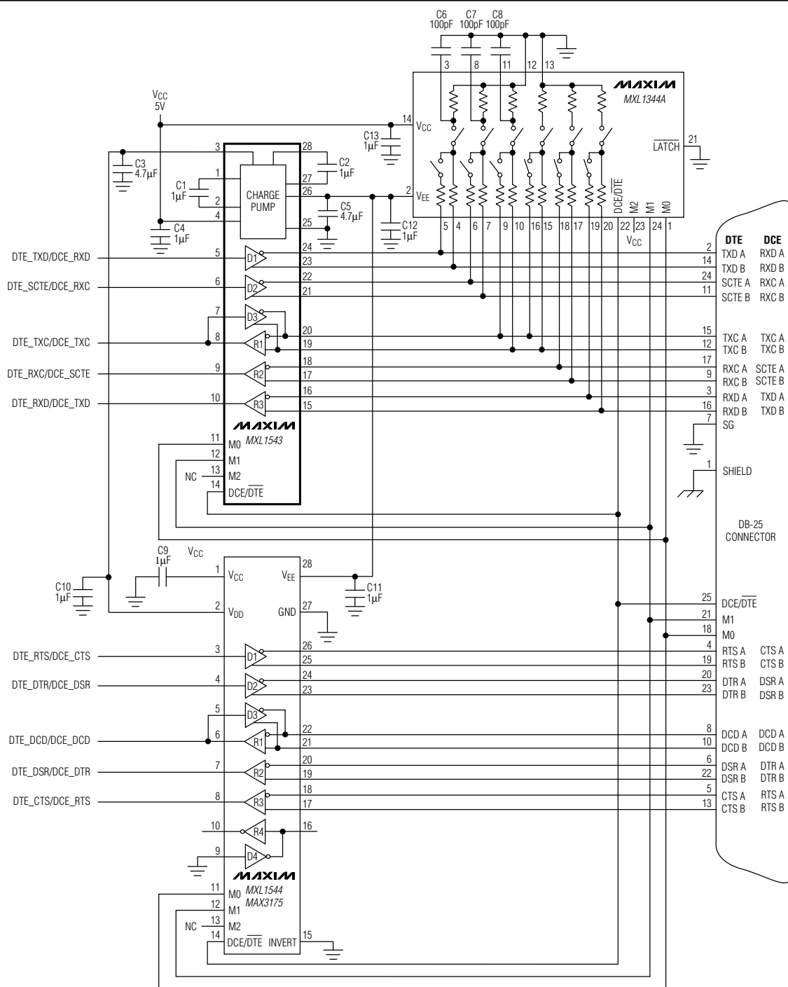
Figure 11. Cable-Selectable Multiprotocol DTE/DCE Port
