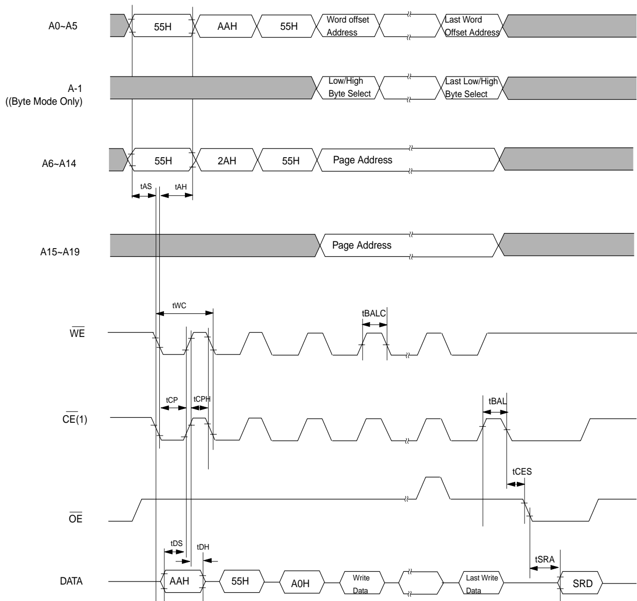
Figure 14. AUTOMATIC PAGE PROGRAM TIMING WAVEFORM(Alternate \overline{CE} Controlled)
