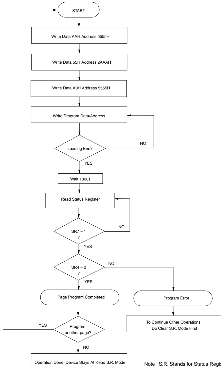
Figure 1. AUTOMATIC PAGE PROGRAM FLOW CHART
