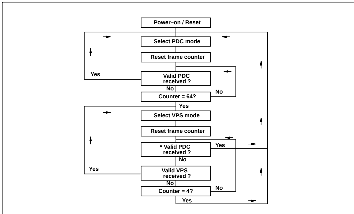
Fig. 6 Flow chart of VPS/PDC Switching
