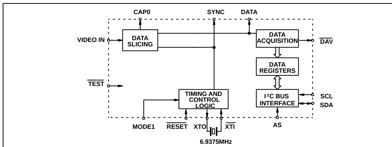
Fig. 2 MV1821 block diagram
