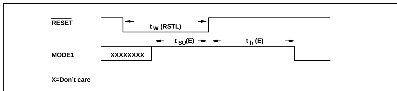
Fig. 3 VPS ONLY mode timing
