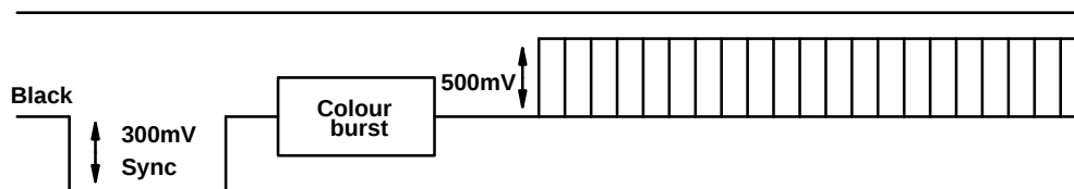
Fig. 5 Waveforms of Video Data
