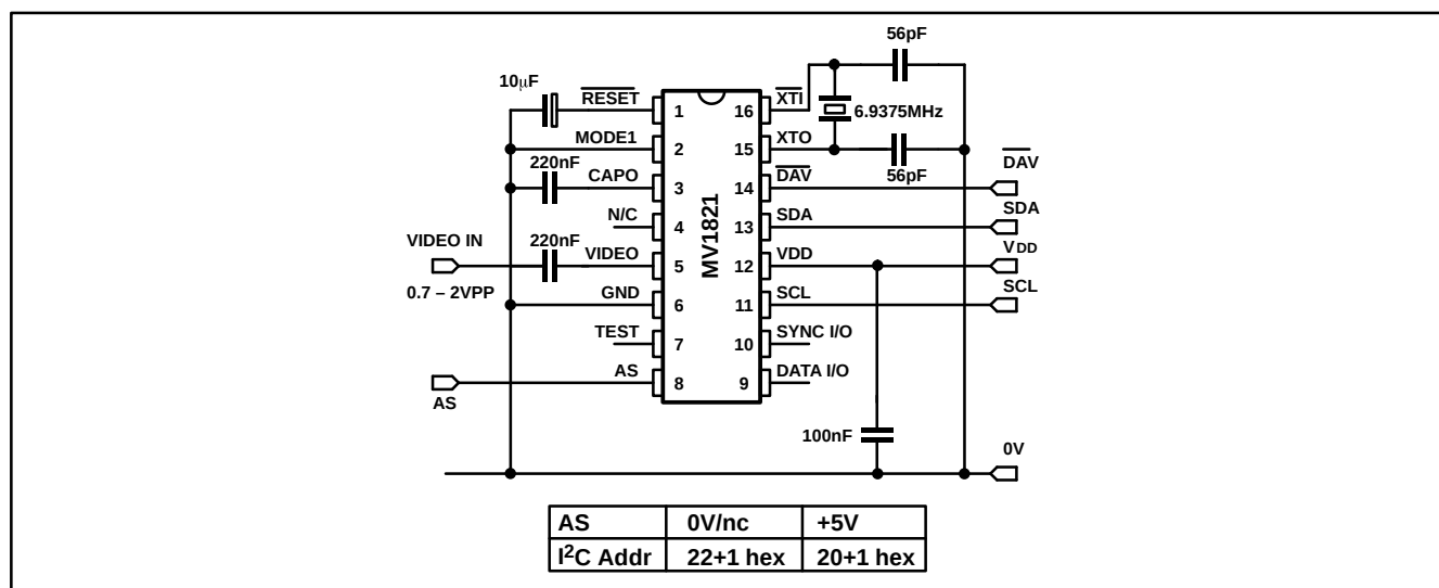
Fig. 4. Typical application diagram
