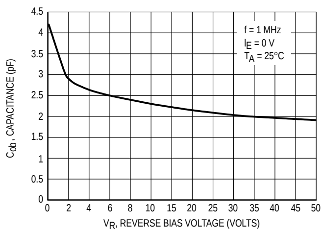
Figure 39. Output Capacitance
