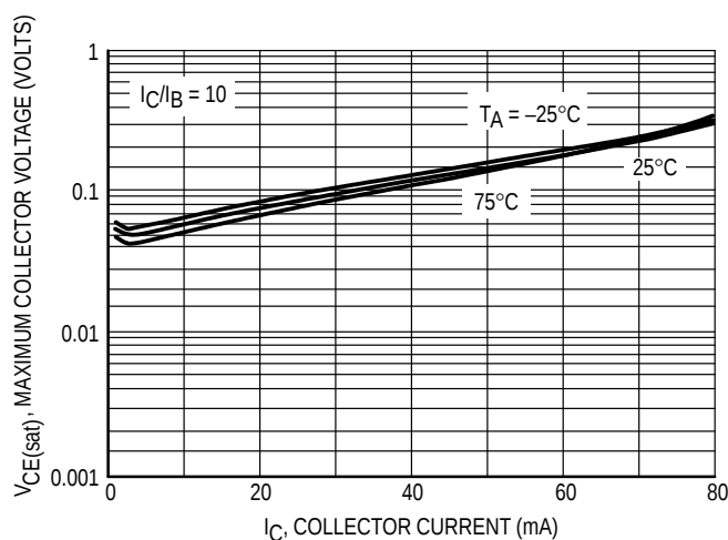
Figure 37. V_{CE(sat)} versus I_C
