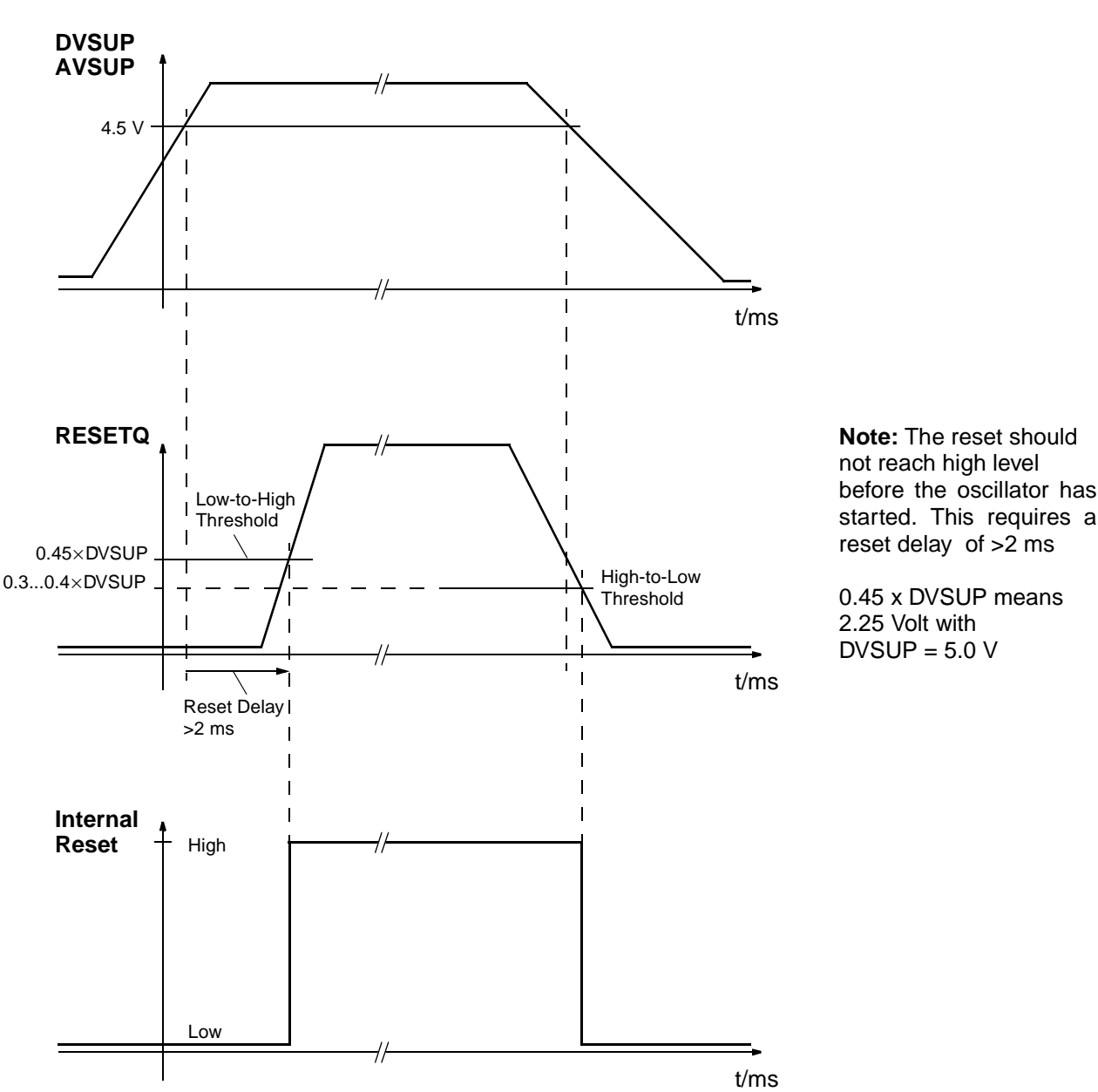
Fig. 4–22: Power-up sequence
