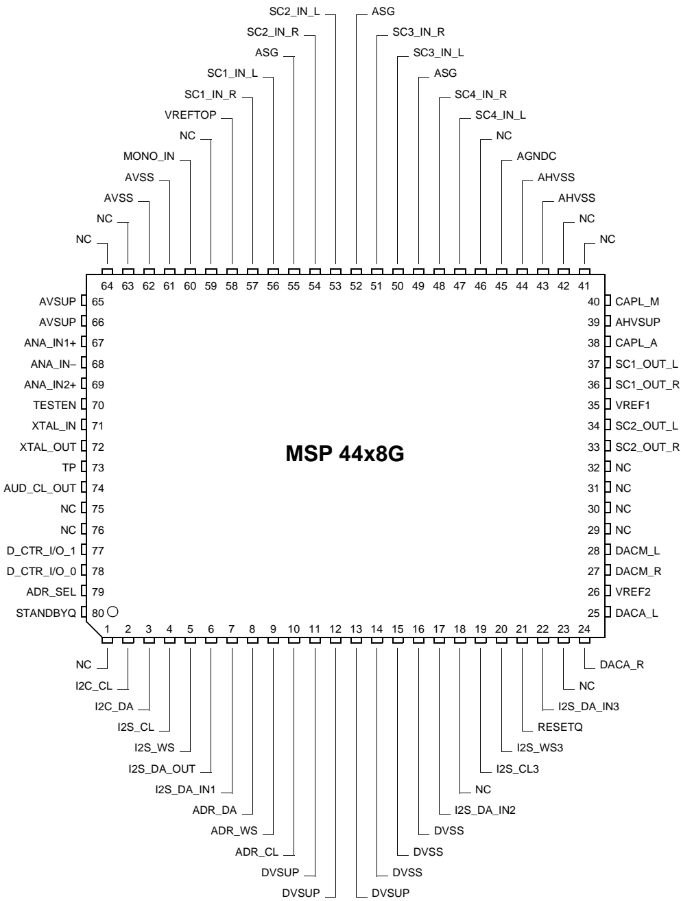
Fig. 4–4: PQFP80 package
