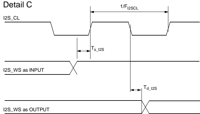
Fig. 4–24: I 2 S timing diagram (synchronous interface)
