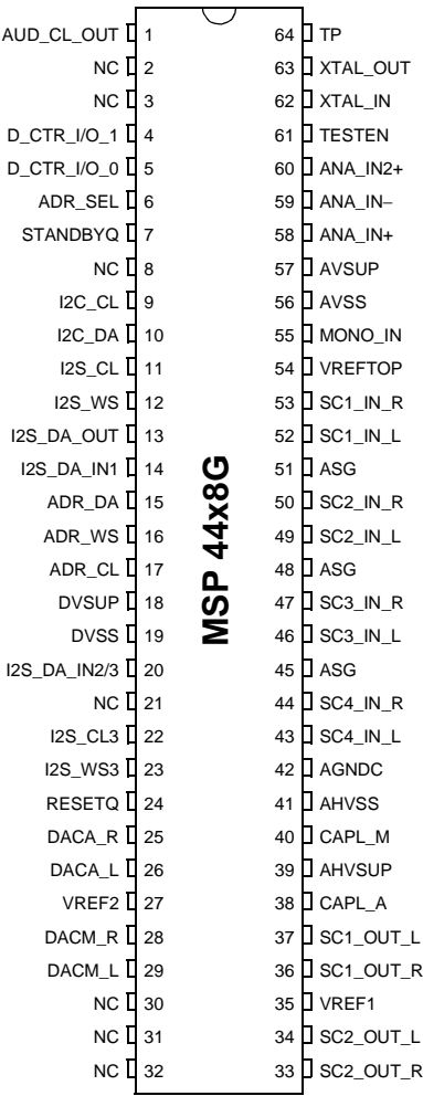
Fig. 4–6: PSDIP64 package
