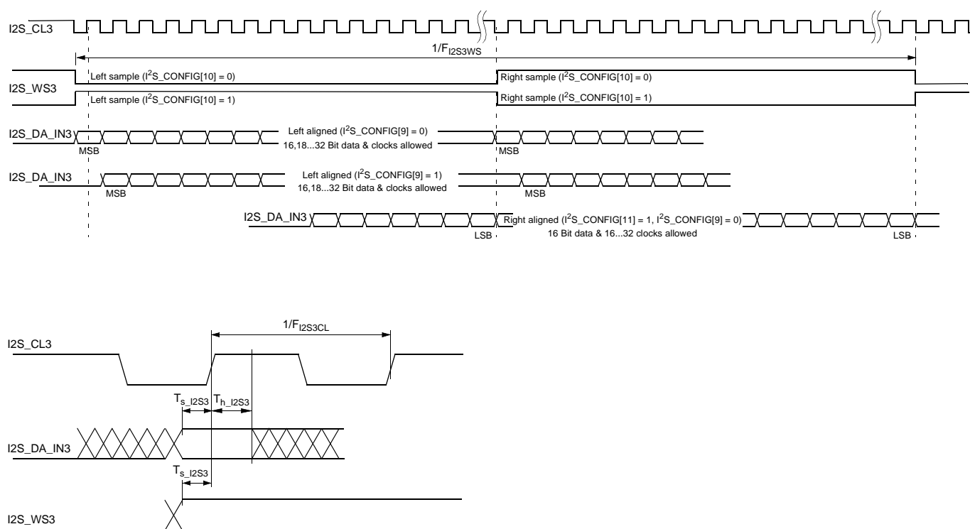
Fig. 4-25: I²S timing diagram (asynchronous interface)
