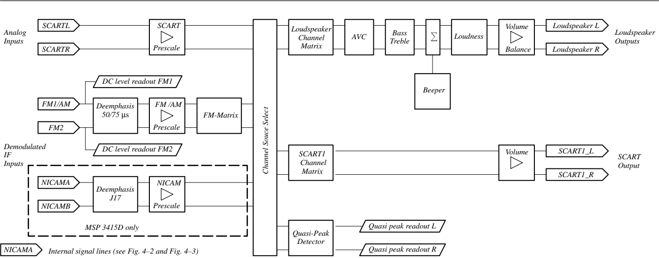
Fig. 4–5: Audio Baseband Processing (DSP-Firmware)
