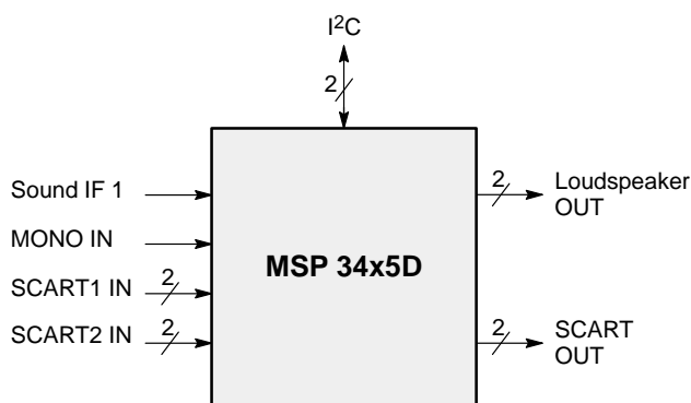
Fig. 1–1: Main I/O Signals MSP 34x5D
