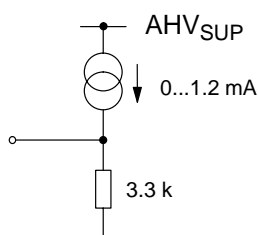
Fig. 8-20: Output Pins 56, 57 (DACM_L/R)
