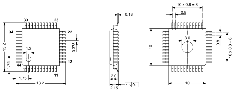
Fig. 8-5: 44-Pin Plastic Quad Flat Package (PQFP44) Weight approx. 0.4 g Dimensions in mm
