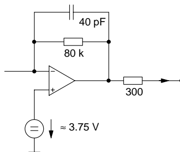
Fig. 8-19: Output Pins 47, 48 (SC1_OUT_L/R)
