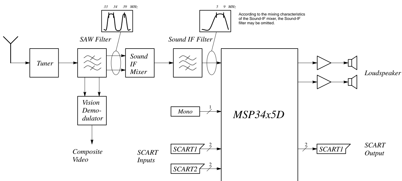
Fig. 3–1: Typical MSP 34x5D application
