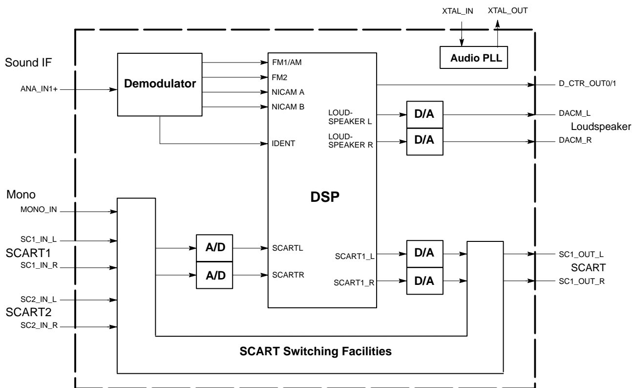
Fig. 4–1: Architecture of the MSP 34x5D
