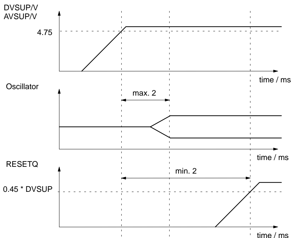
Fig. 5–3: Power-up sequence
