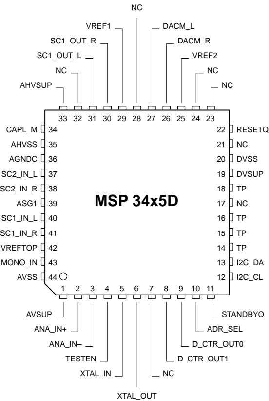
Fig. 8–10: 44-pin PQFP package
