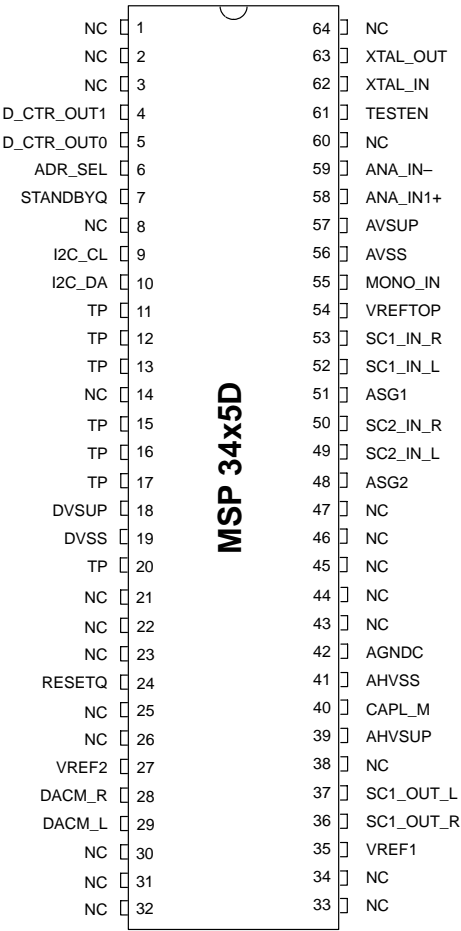
Fig. 8-7: 64-pin PSDIP package
