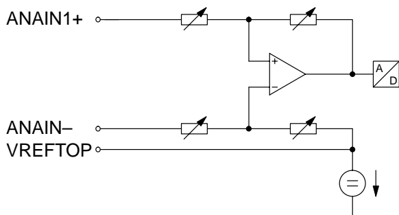
Fig. 8-14: Input Pins 24, 25, and 29 (ANA_IN-, ANA_IN1+, VREFTOP)
