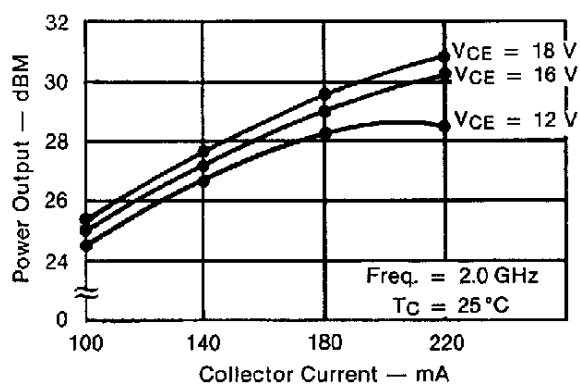
TYPICAL POWER OUTPUT &amp; GAIN @ 1dB COMPRESSION POINT vs COLLECTOR CURRENT
