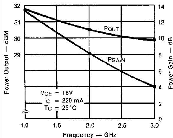
TYPICAL POWER OUTPUT &amp; GAIN @ 1dB COMPRESSION POINT vs FREQUENCY
