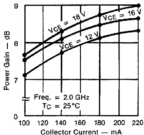
TYPICAL LINEAR GAIN vs COLLECTOR CURRENT
