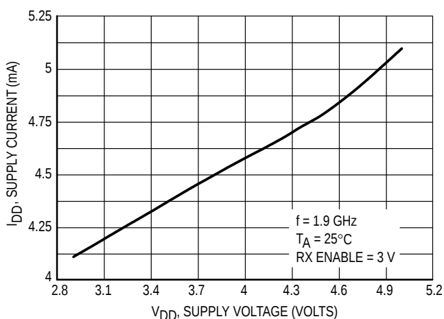
Figure 7. Supply Current versus Voltage
