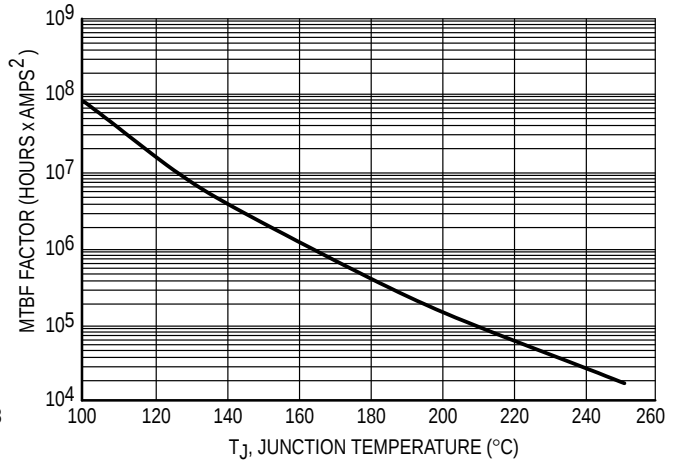
Figure 10. MTBF Factor versus Junction Temperature
