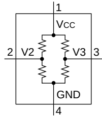
Magneto-Sensing Element -Equivalent Circuit-
