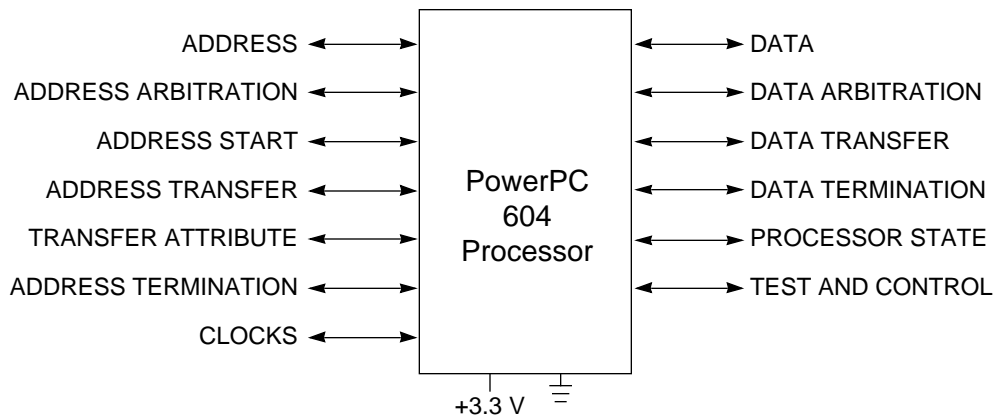
Figure 4. System Interface
