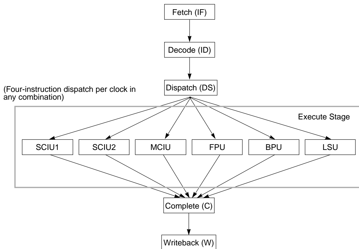
Figure 7. Pipeline Diagram
