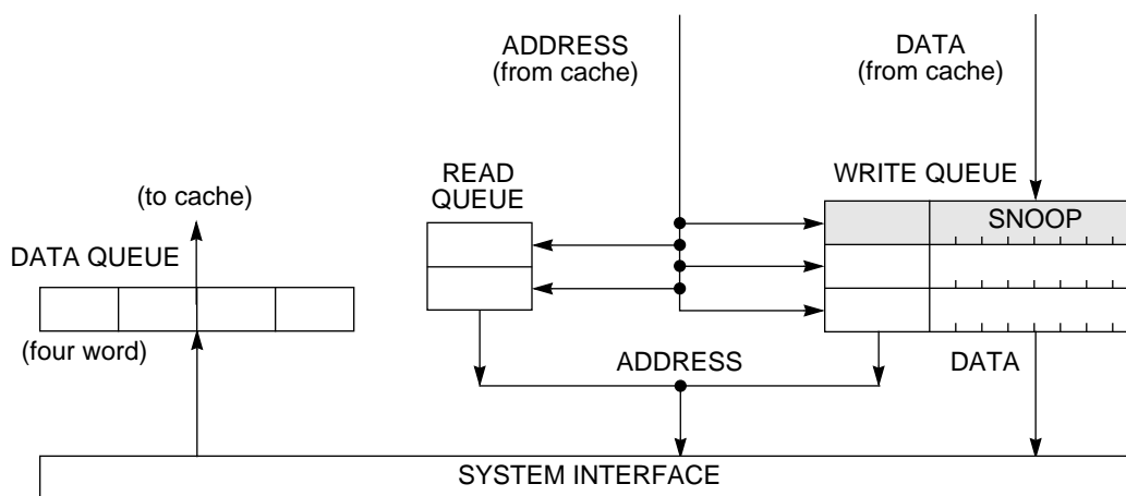
Figure 2. Memory Unit
