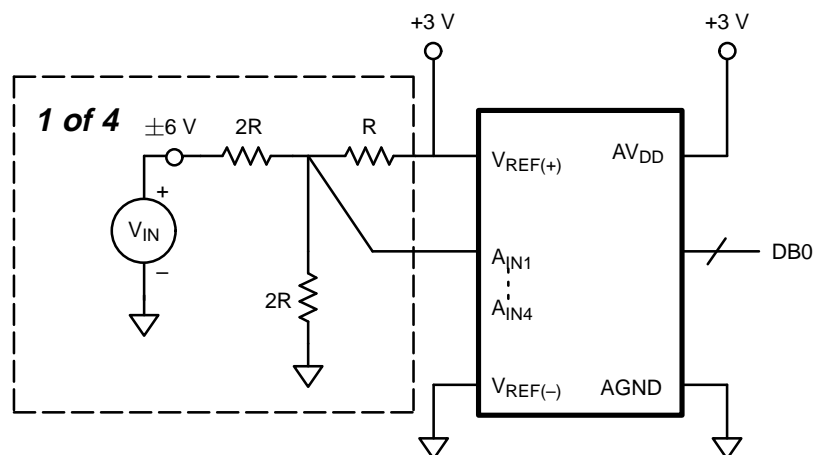
Figure 16. \pm 3 V Analog Input
