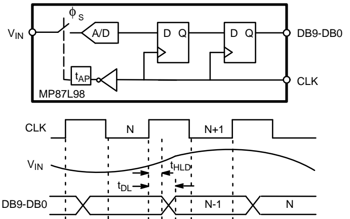
Figure 12. MP87L98 Functional Equivalent Circuit and Interface Timing
