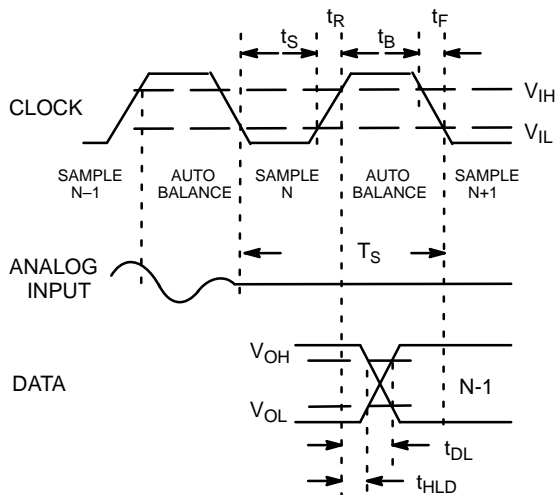
Figure 1. MP87L98 Timing Diagram
