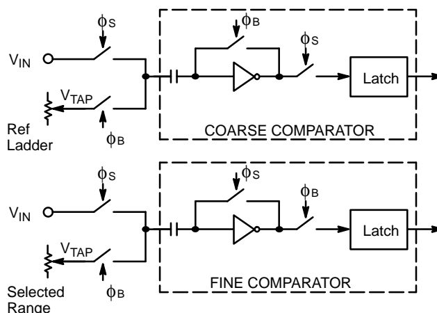
Figure 2. MP8798 Comparators
