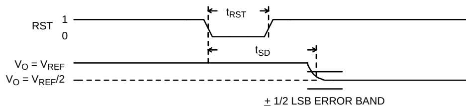
Figure 3. RESET Operation
