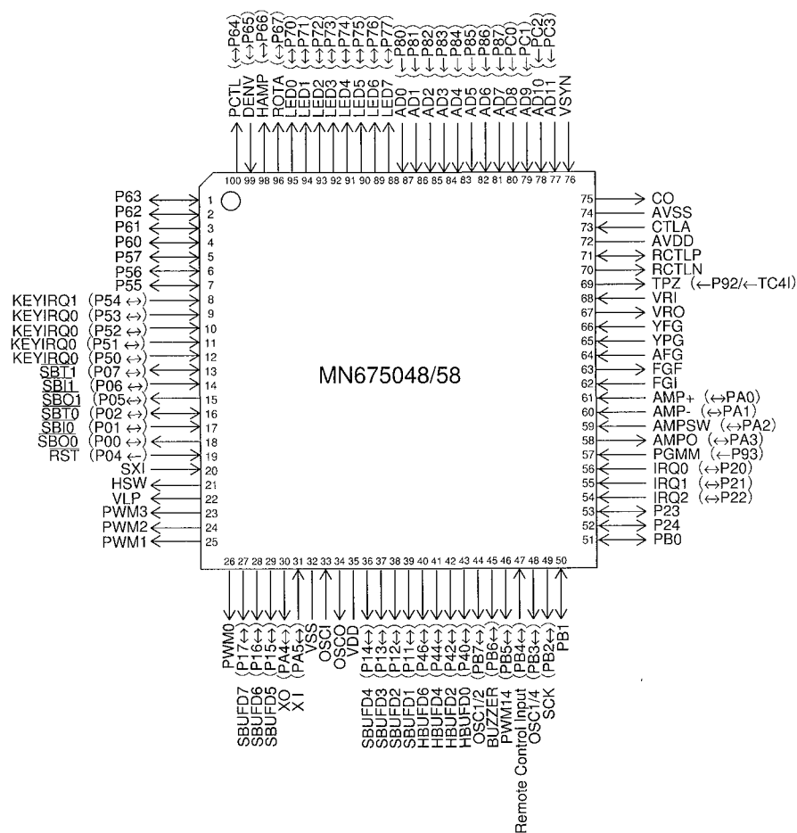
QFP100-P-1818 / QFP100-P-1818B
