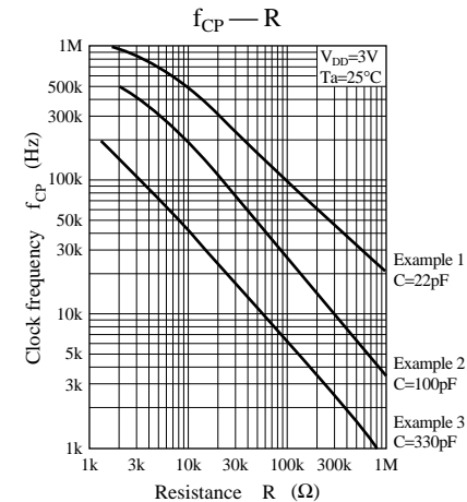
Fig.1 Example of Clock Oscillation Frequency Characteristics
