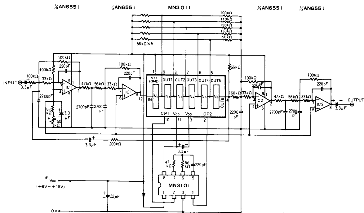
Reverberation Effect Generation Circuit
