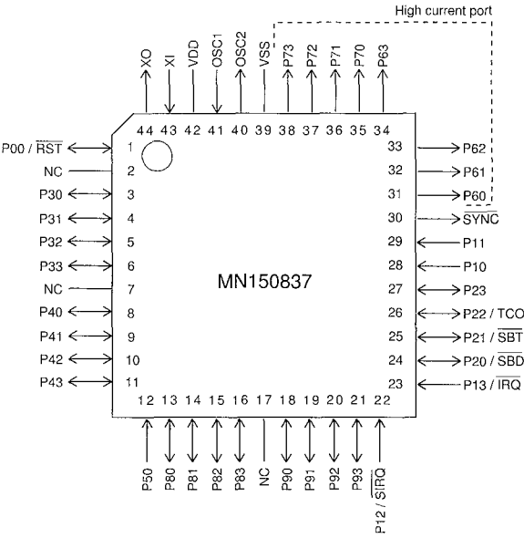
QFP044-P-1010
