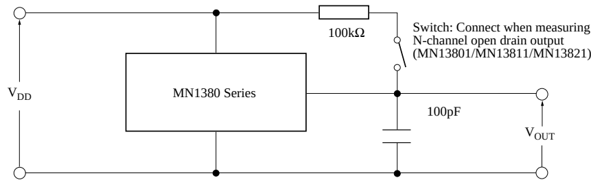
Figure 3. Circuit for Measuring the Output Characteristics
