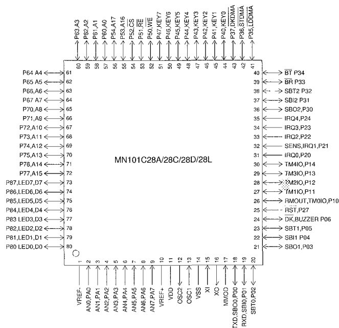
LQFP080-P-1414A (MN101C28A / 28C / 28D / 28L)
