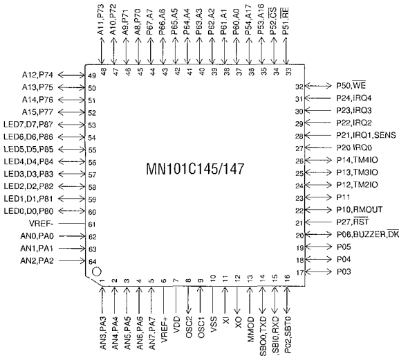
LQFP064-P-1414
