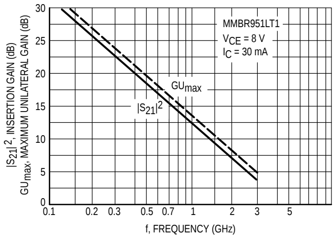
Figure 6. MMBR951LT1
