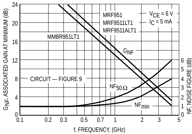
Figure 7. Typical Noise Figure and Associated Gain versus Frequency
