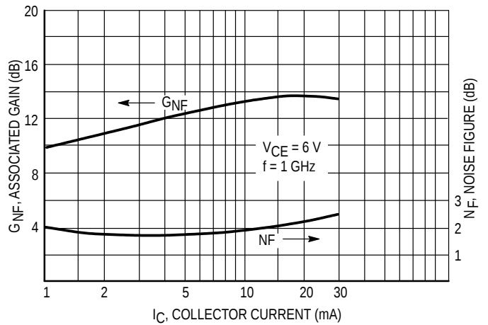
Figure 17. Associated Gain versus Collector Current
