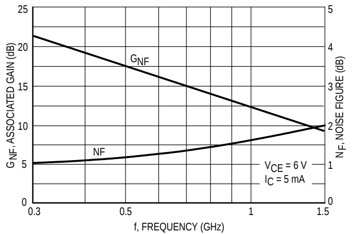
Figure 19. Noise Figure and Associated Gain versus Frequency
