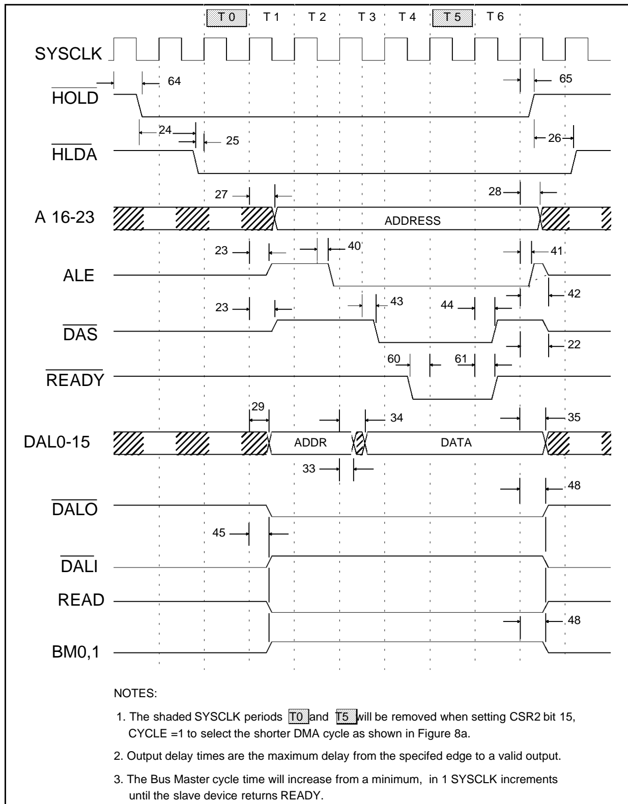
Figure 12: MK50H28 BUS Master Timing Diagram (Write) (for CYCLE = 0, CSR2&lt;15&gt;)
