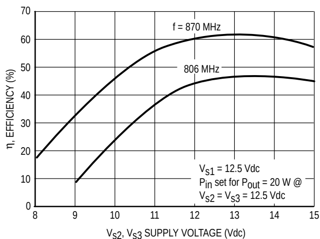
Figure 5. Efficiency versus Supply Voltage
