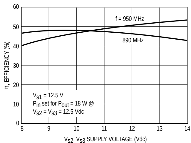
Figure 11. Efficiency versus Supply Voltage
