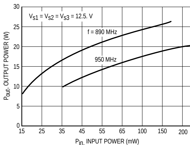
Figure 9. Output Power versus Input Power
