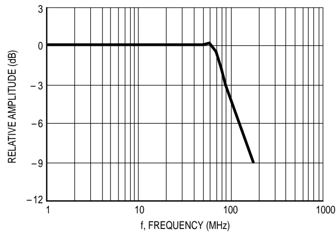
Figure 3. Frequency Response
