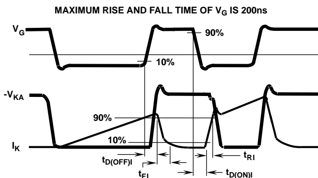
FIGURE 17. SWITCHING TEST WAVEFORMS
