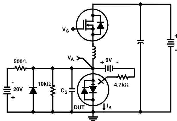
FIGURE 16. V_{SPIKE} TEST CIRCUIT
