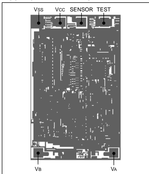
FIGURE 3-1: DIE PLOT
