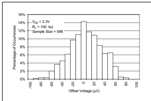
FIGURE 2-3: Histogram of Offset Voltage with V_{DD} = 2.3\text{V} .
