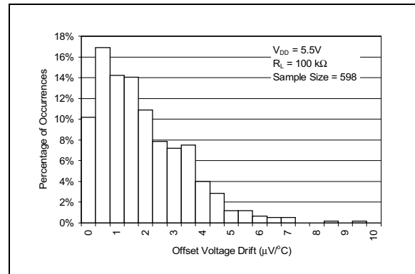
FIGURE 2-2: Histogram of Offset Voltage Drift with V_{DD} = 5.5\text{V} .
