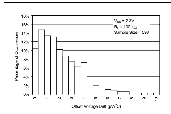
FIGURE 2-4: Histogram of Offset Voltage Drift with V_{DD} = 2.3\text{V} .
