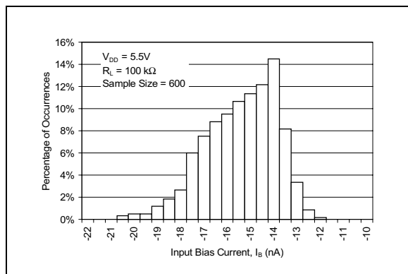
FIGURE 2-5: Histogram of Input Bias Current with V_{DD} = 5.5\text{V} .
