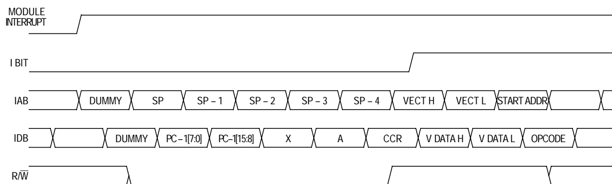
Figure 6-8. Interrupt Entry
