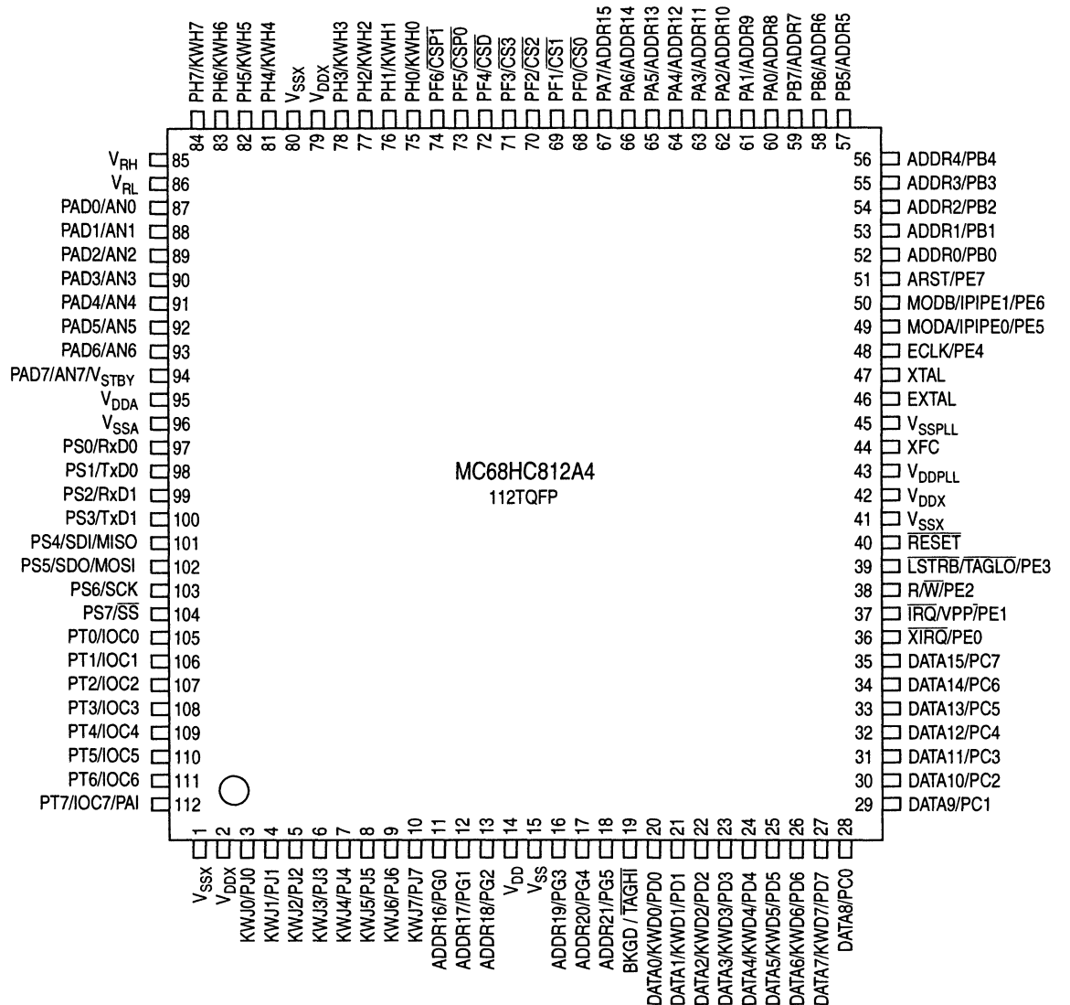
Figure 3 Pin Assignments for MC68HC812A4
