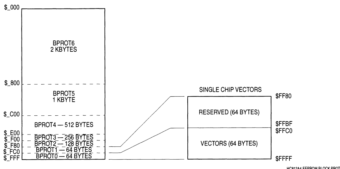
Figure 5 EEPROM Block Protect Mapping
