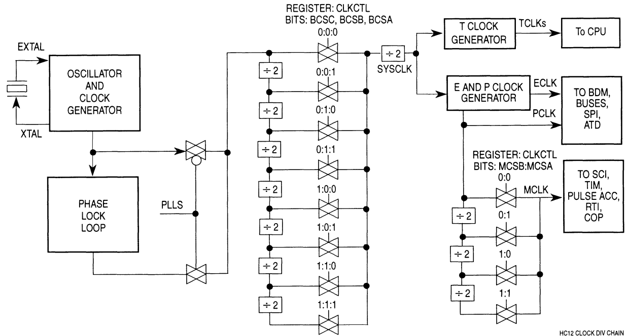
Figure 13 Clock Divider Chain
