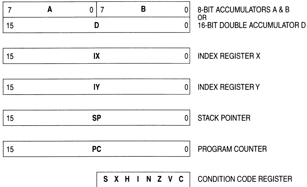
Figure 2 Programming Model
