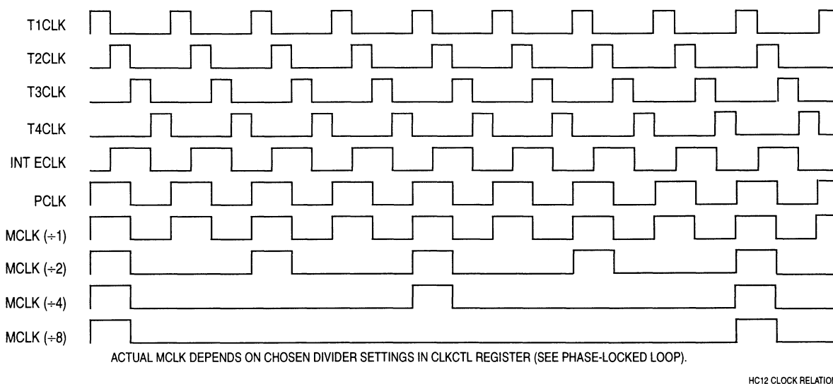
Figure 12 Internal Clock Relationships
