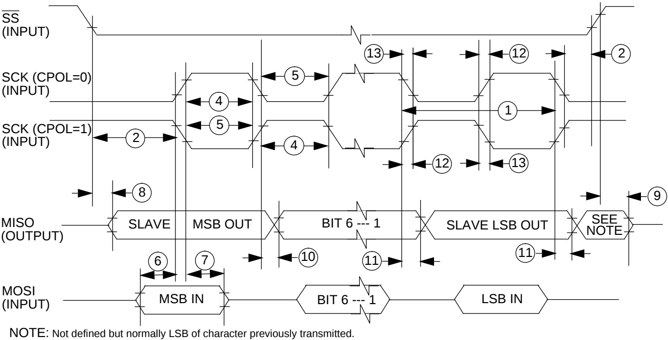
Figure 17-3: SPI SLAVE TIMING (CPHA = 0)
