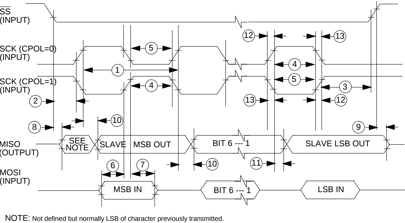
Figure 17-4: SPI SLAVE TIMING (CPHA = 1)
