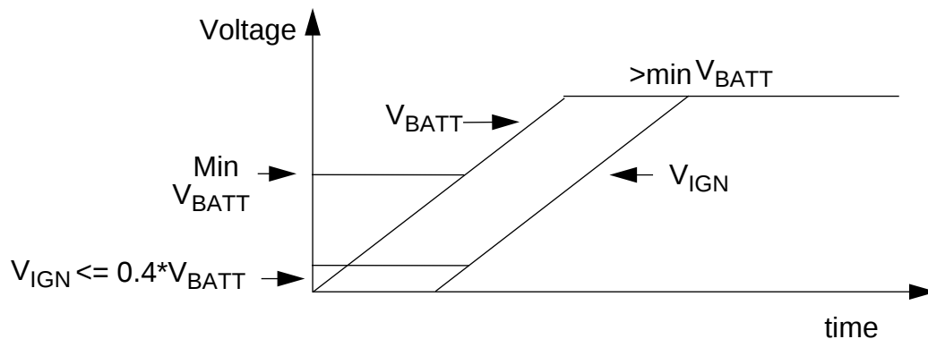
Figure 7-3: Regulator Startup
