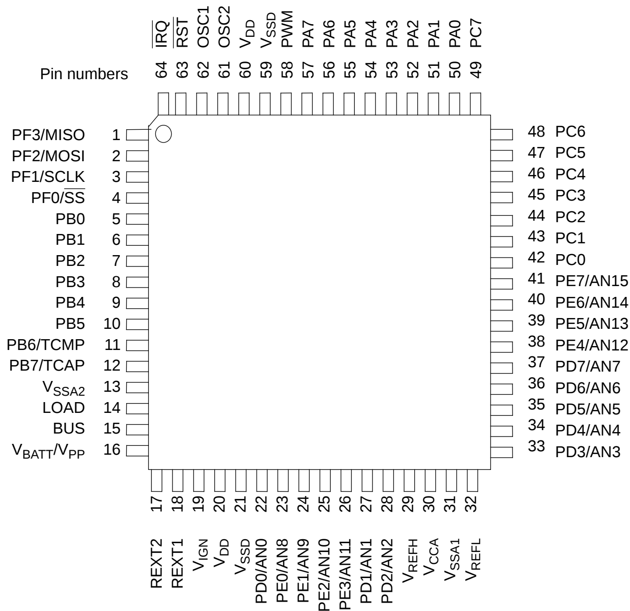
Figure 1-3: MC68HC705V8 Pin Assignments (64-pin QFP)
