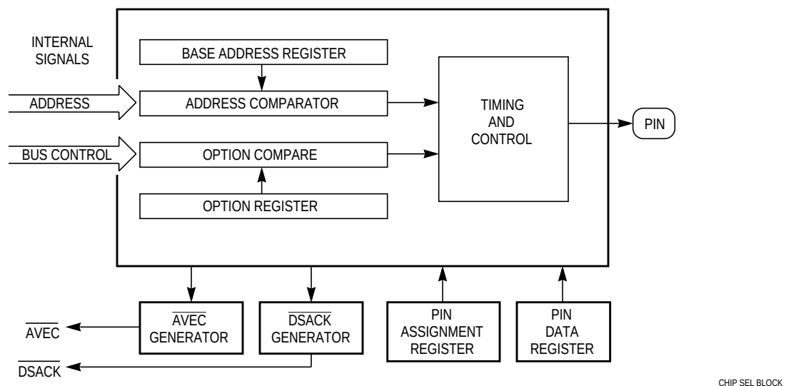
Figure 5-22 Chip-Select Circuit Block Diagram
