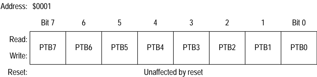
Figure 11-5. Port B Data Register (PTB)
