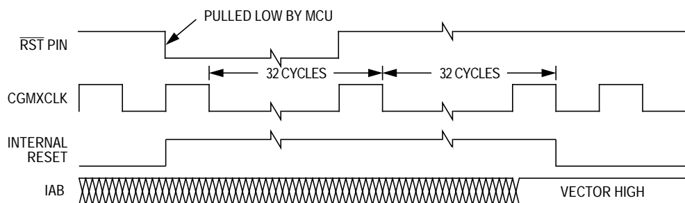
Figure 6-3. Active Reset Recovery Timing
