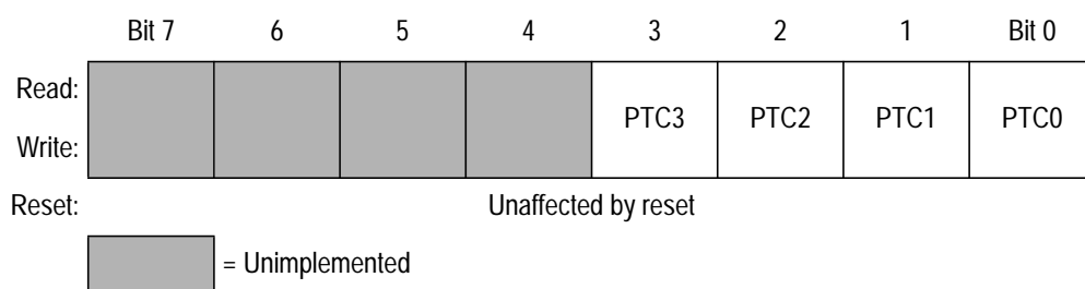
Figure 11-8. Port C Data Register (PTC)
