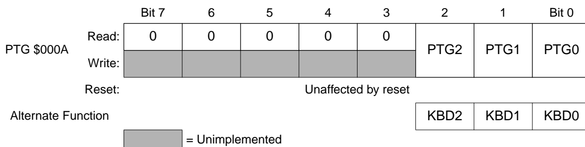
Figure 19. Port G data register (PTG)
