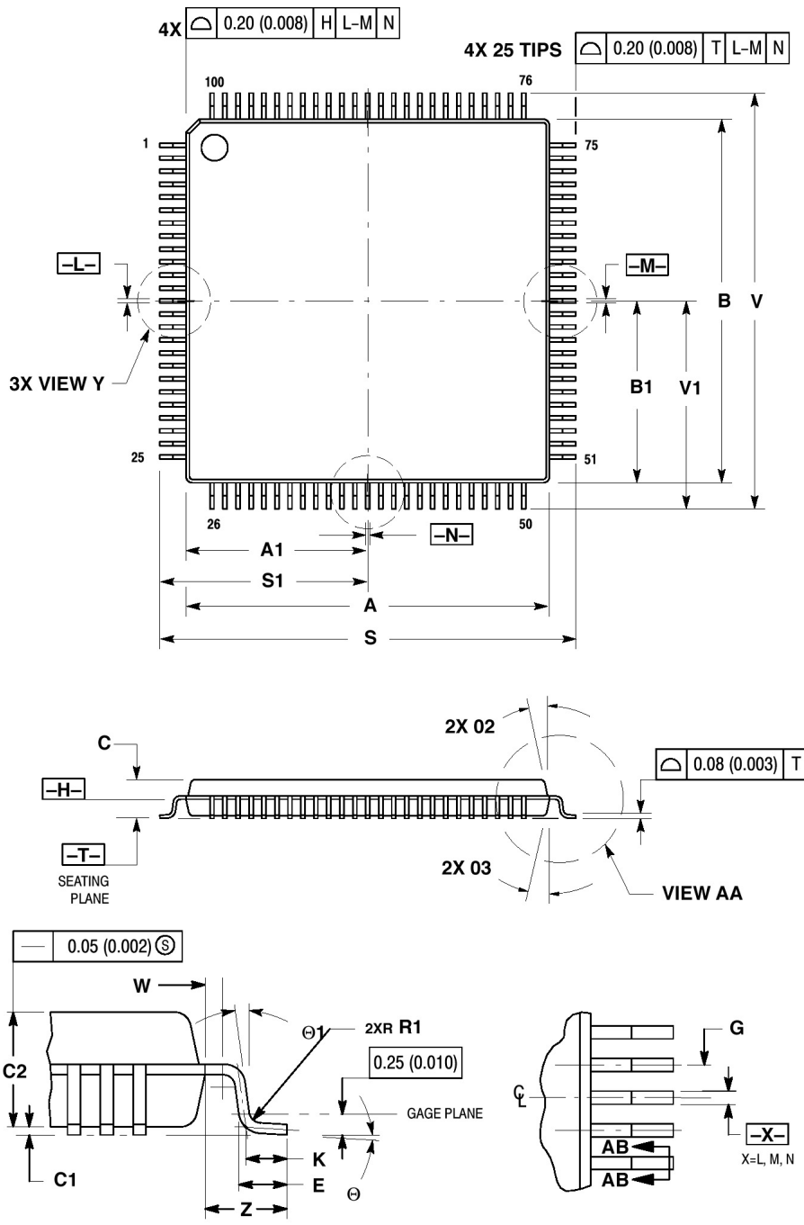
Figure 7. 100-pin QFP
