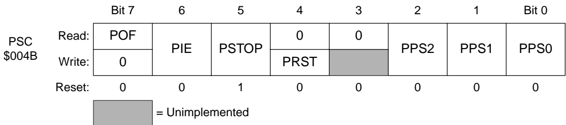
Figure 2. PIT Status and Control Register (TSC)
