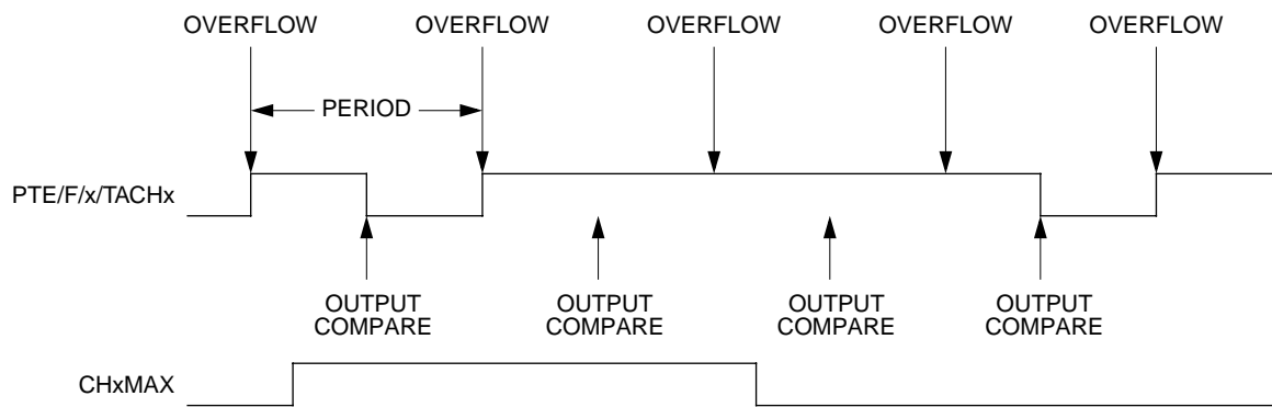
Figure 7. CHxMAX Latency
