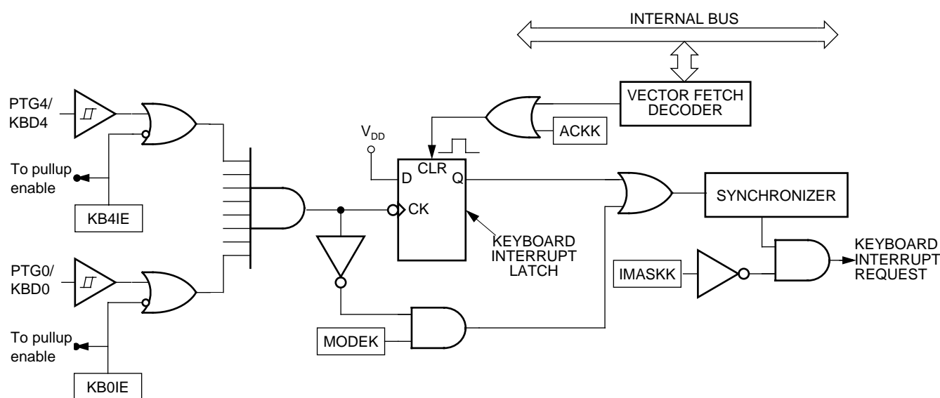
Figure 5. Keyboard module block diagram
