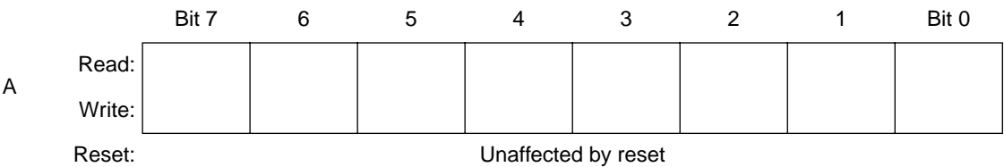
Figure 1. Accumulator (A)
