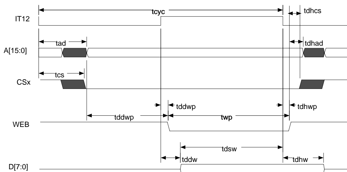
Figure 4 High performance write timings
