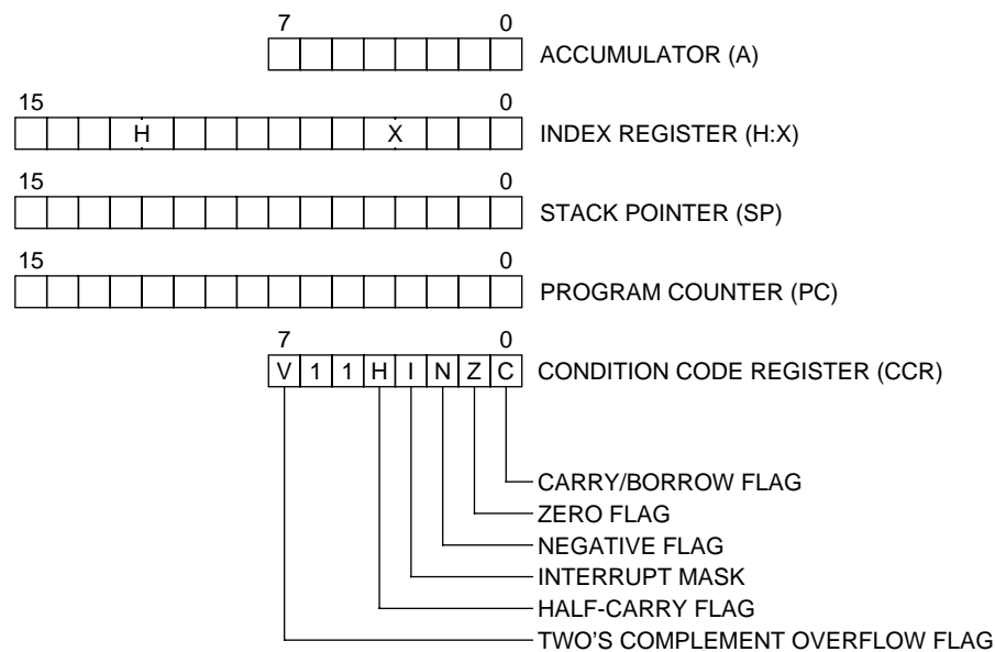
Figure 1. CPU registers
