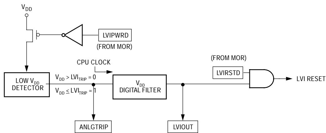
Figure 1. LVI module block diagram
