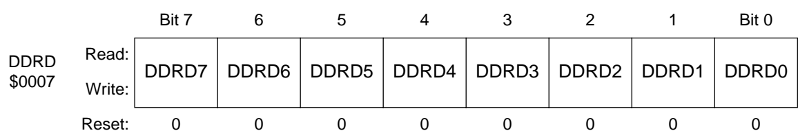
Figure 11. Data direction register D (DDRD)
