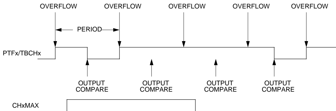
Figure 15. CHxMAX latency
