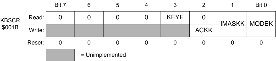
Figure 6. Keyboard status and control register (KBSCR)
