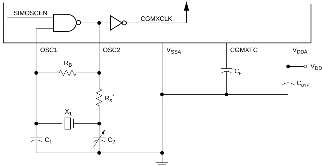
Figure 9-3. CGM External Connections
