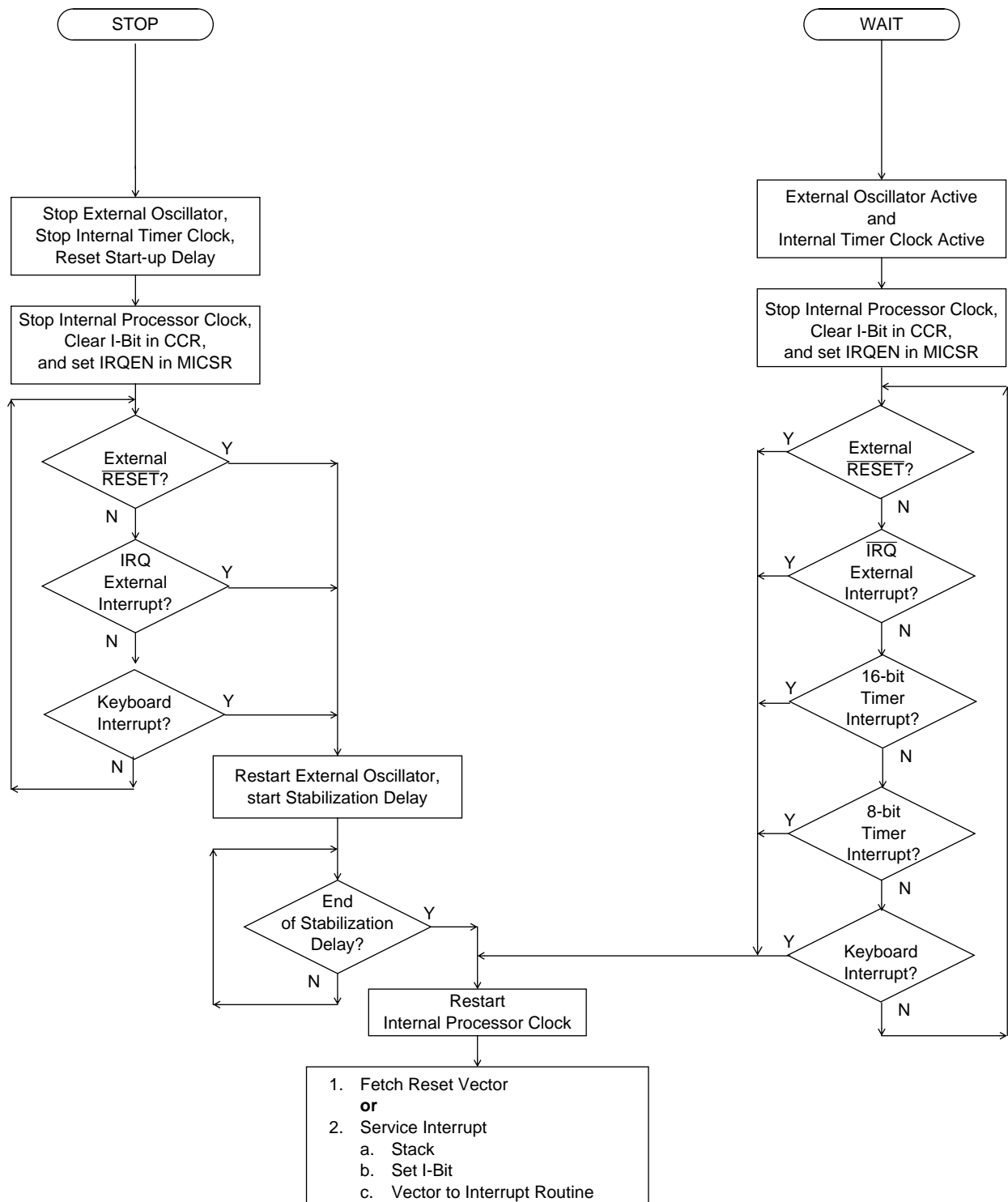
Figure 6-1. STOP/WAIT Flowchart
