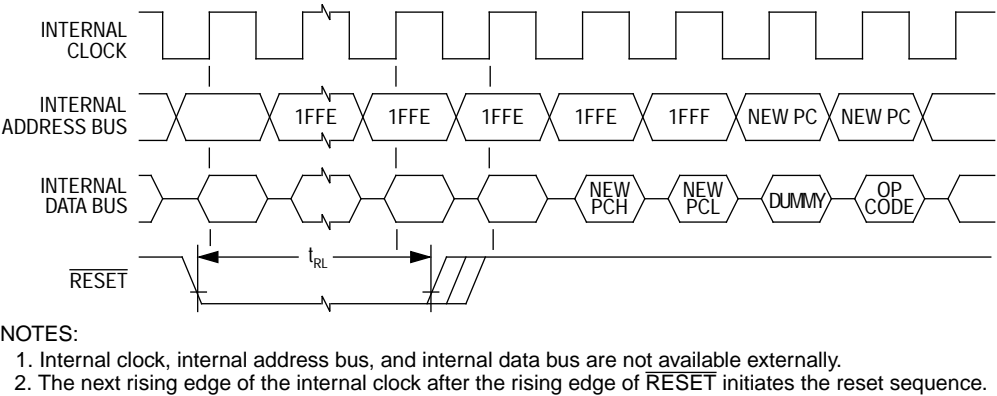
Figure 19. External Reset Timing
