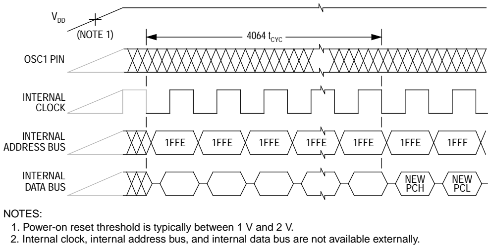
Figure 18. Power-On Reset Timing
