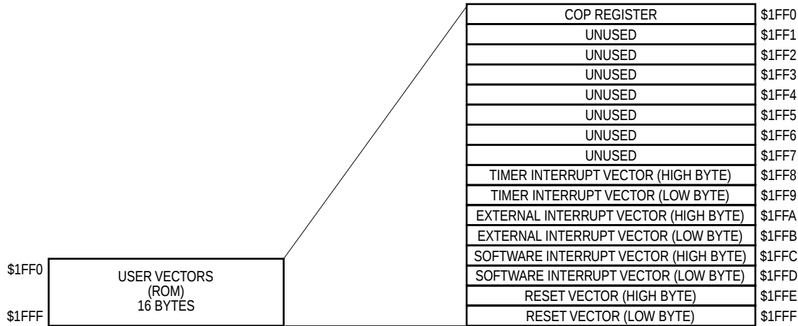
Figure 2-1. Memory Map
