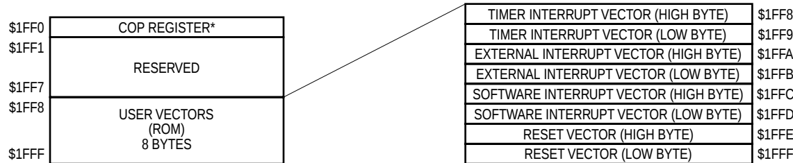
Figure 2-1. Memory Map
