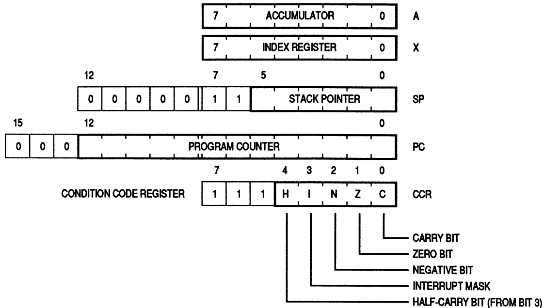
Figure 3-2. Programming Model
