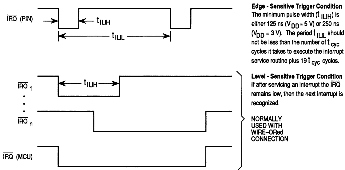
Figure 9-8. External Interrupt Timing
