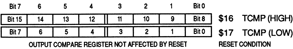
Figure 6-7. Output Compare Register
