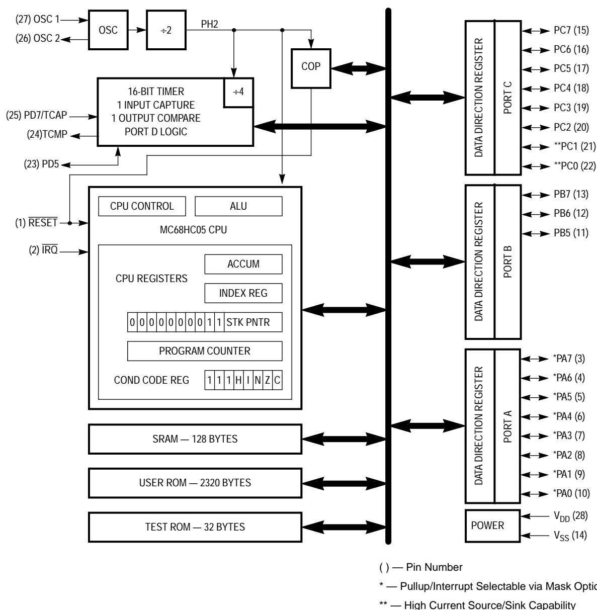
Figure 1-1. MC68HC05P1A Block Diagram
