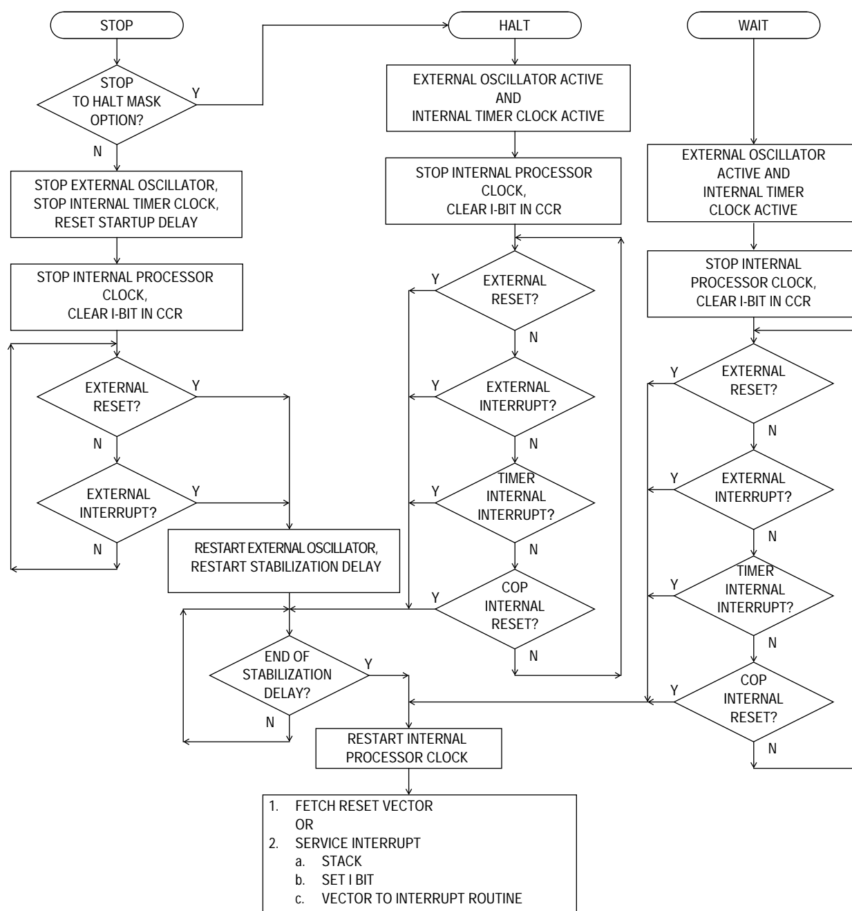
Figure 6-1. STOP/HALT/WAIT Flowchart
