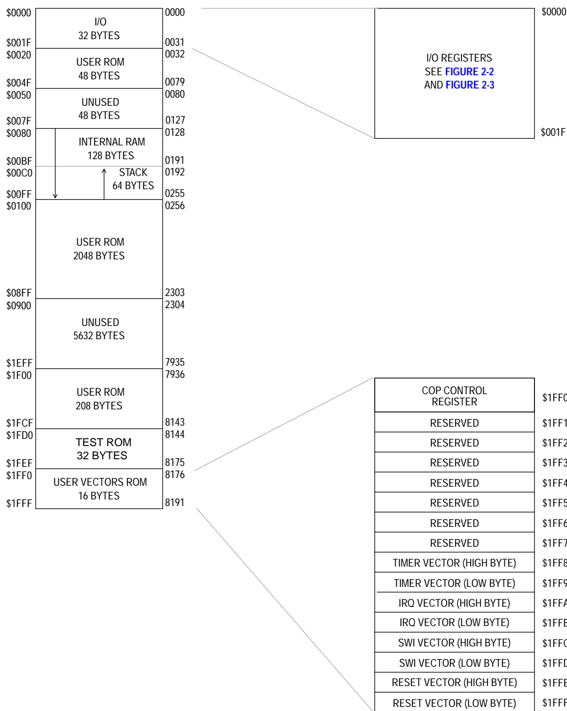
Figure 2-1. Single-Chip Mode Memory Map
