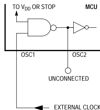
(c) External Clock Source Connections
