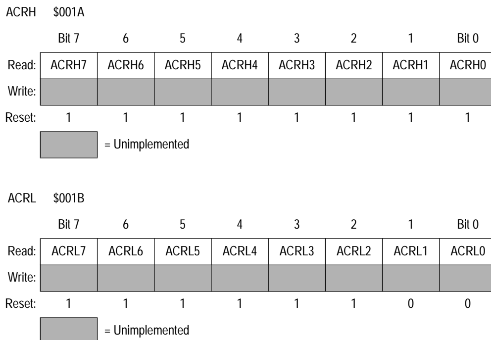
Figure 8-3. Alternate Counter Registers (ACRH/ACRL)
