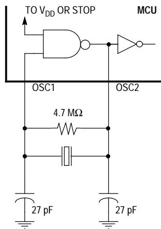
(a) Crystal or Ceramic Resonator Connections
