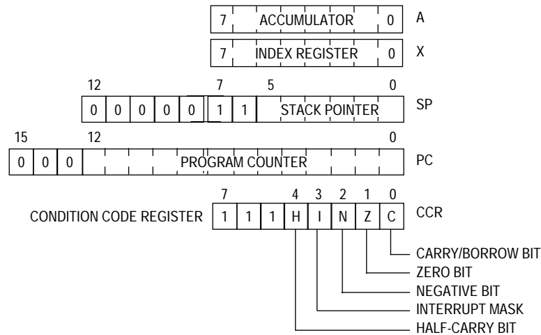
Figure 3-2. Programming Model
