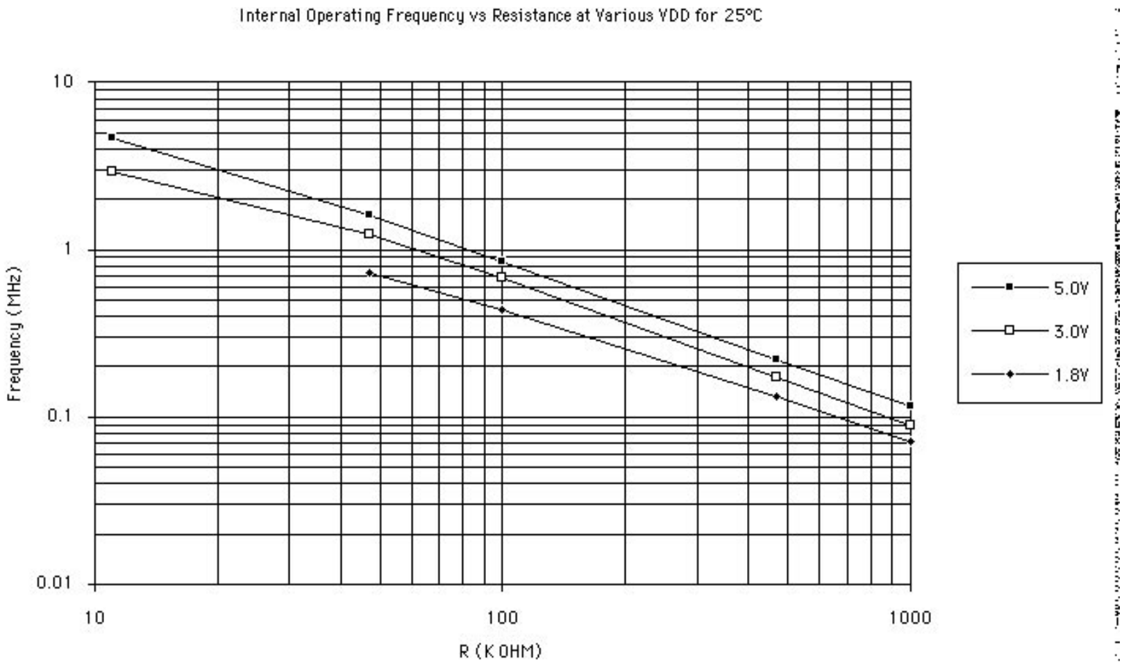
Figure 1-5. Typical Frequency versus Resistance for RC Oscillator Mask Option
