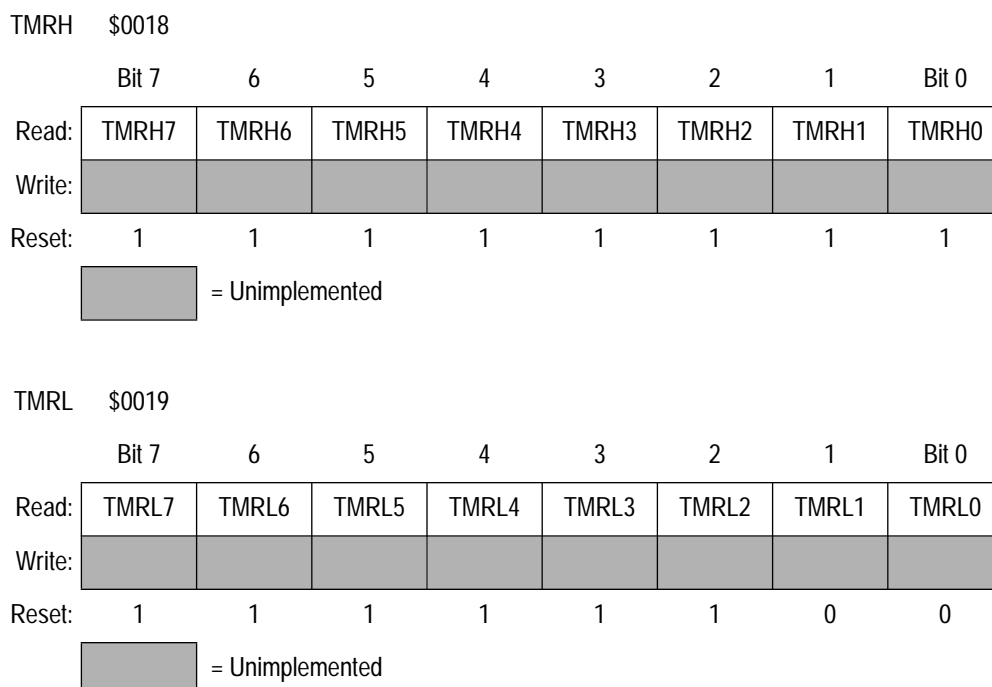
Figure 8-2. Timer Registers (TMRH/TMRL)
