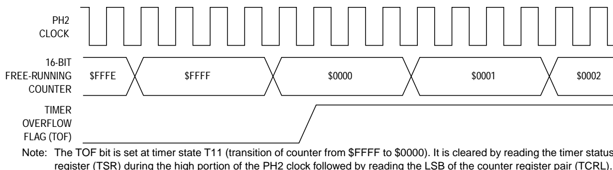
Figure 10-4. State Timing Diagram for Timer Overflow
