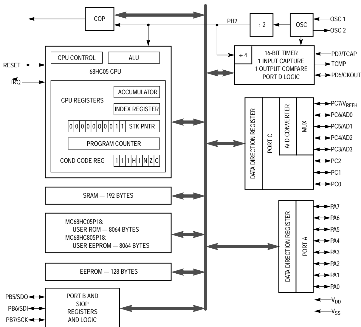
Figure 1-1. MC68HC05P18/MC68HC805P18 Block Diagram
