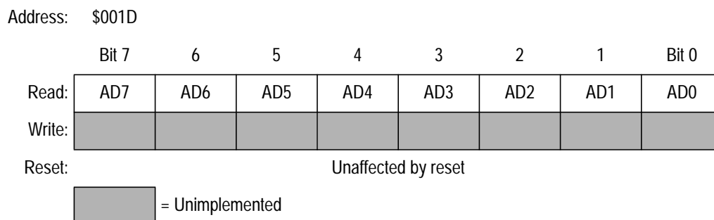
Figure 9-2. A/D Conversion Data Register (ADC)
