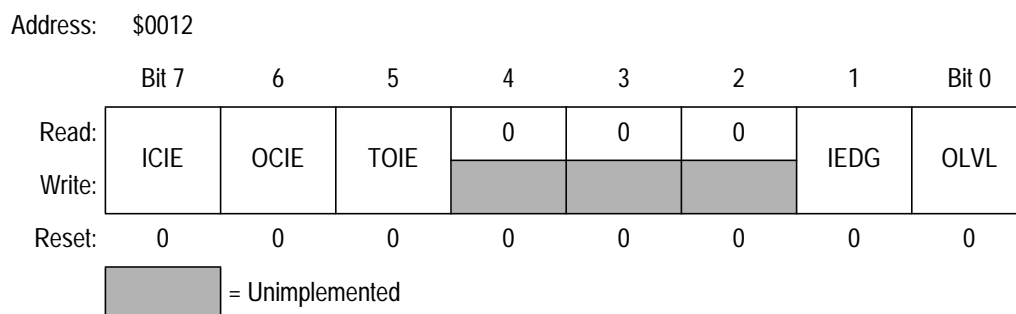
Figure 10-10. Timer Control Register (TCR)
