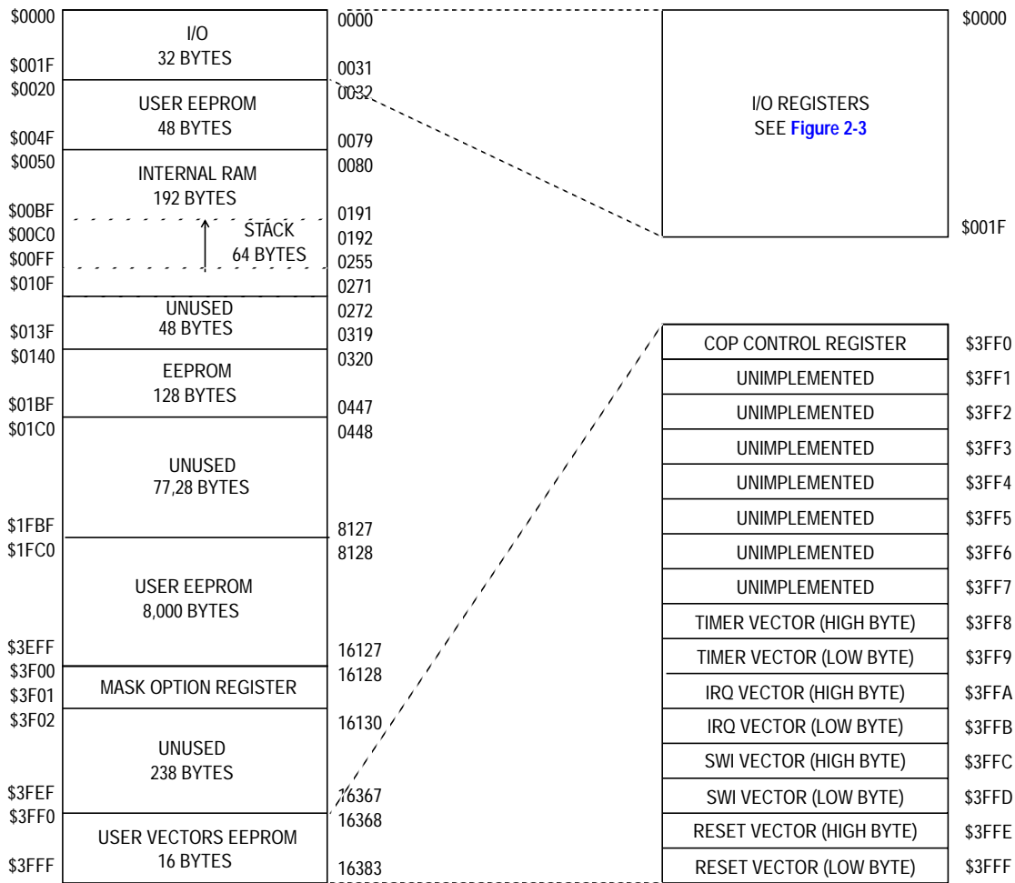
Figure 2-2. MC68HC805P18 User Mode Memory Map
