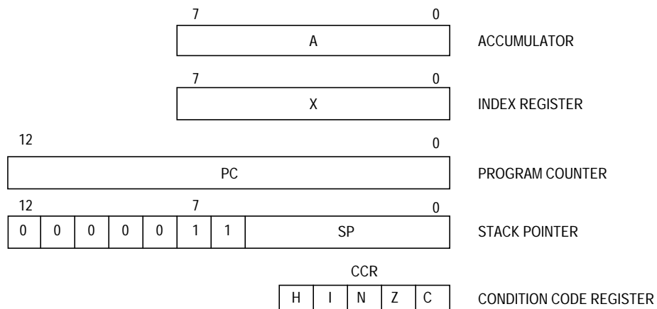
Figure 3-1. Programming Model
