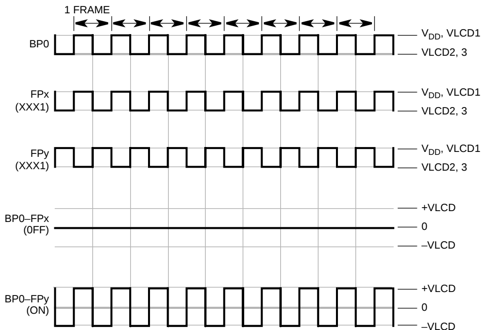
Figure 10-1. LCD 1/1 Duty and 1/1 Bias Timing Diagram
