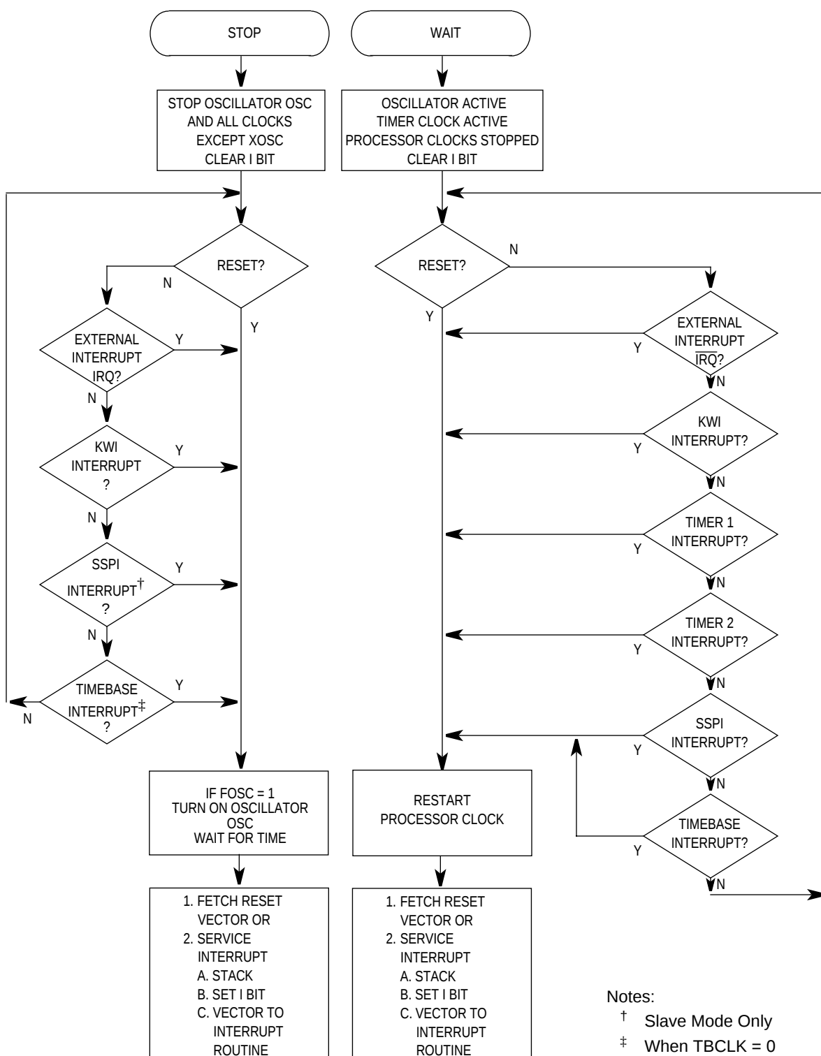
Figure 5-2. Stop/Wait Flowcharts
