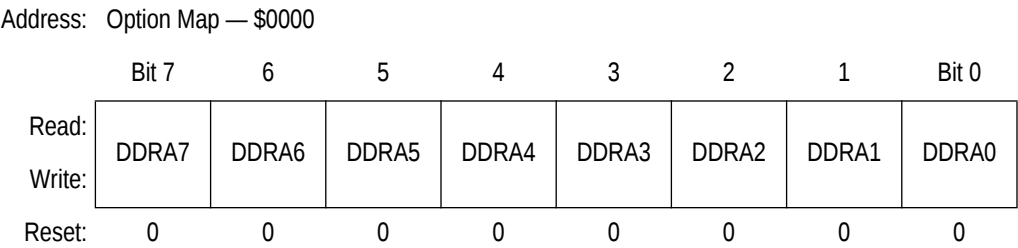
Figure 6-3. Port A Data Direction Register (DDRA)
