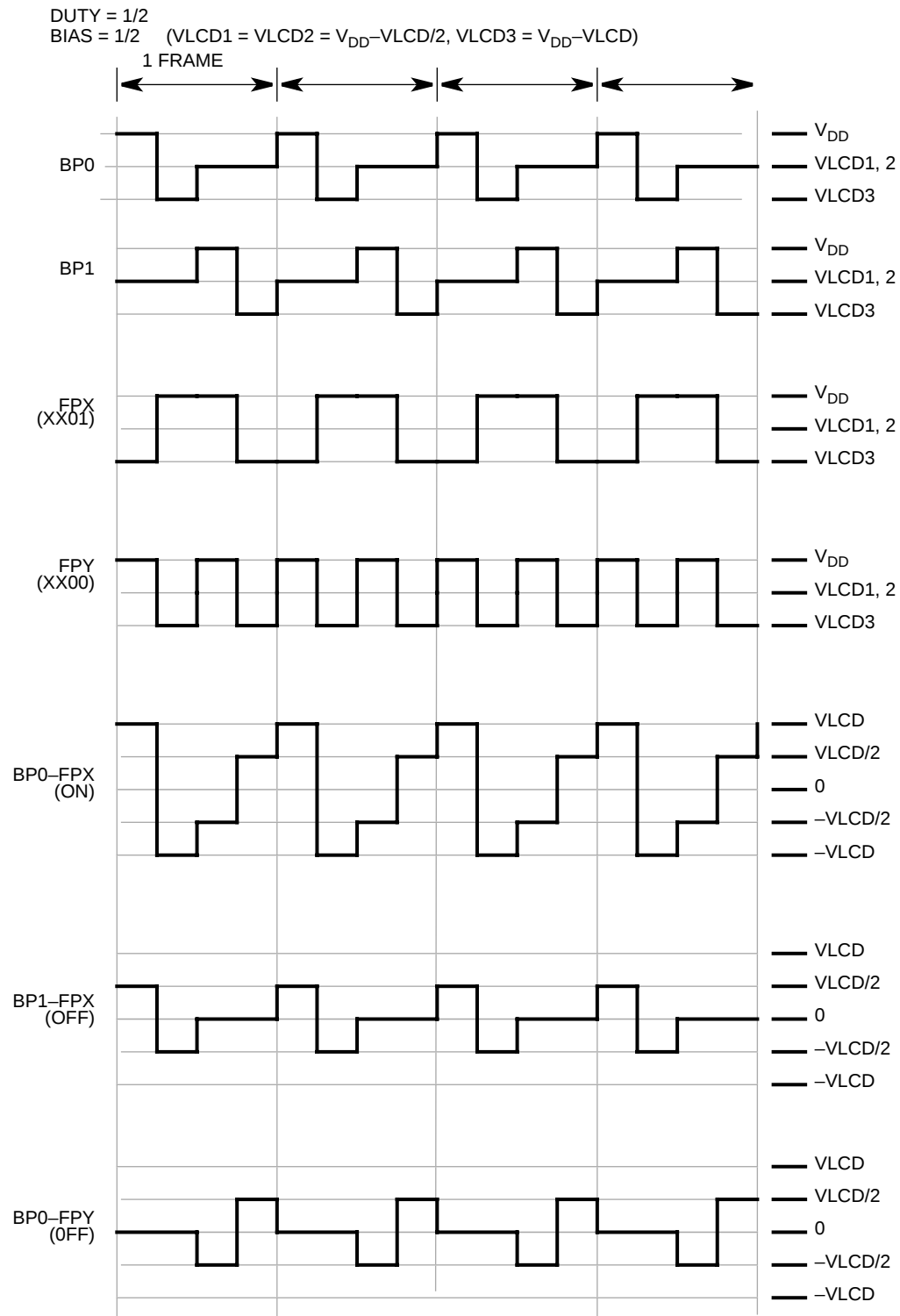
Figure 10-2. LCD 1/2 Duty and 1/2 Bias Timing Diagram
