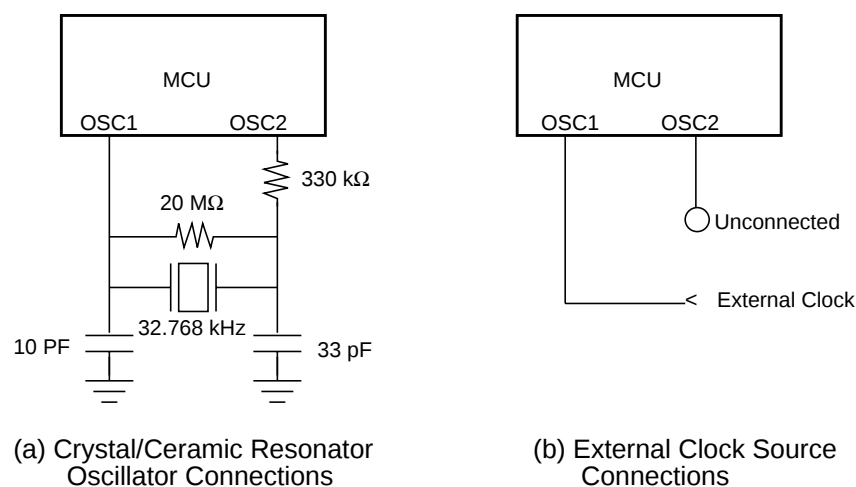
Figure 1-2. Oscillator Connections
