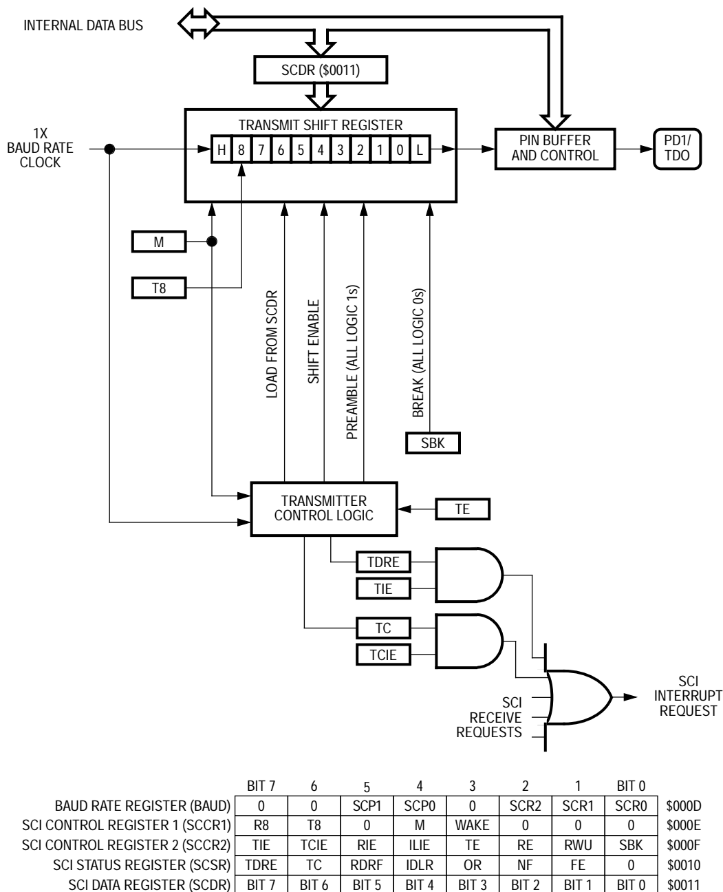
Figure 9-2. SCI Transmitter
