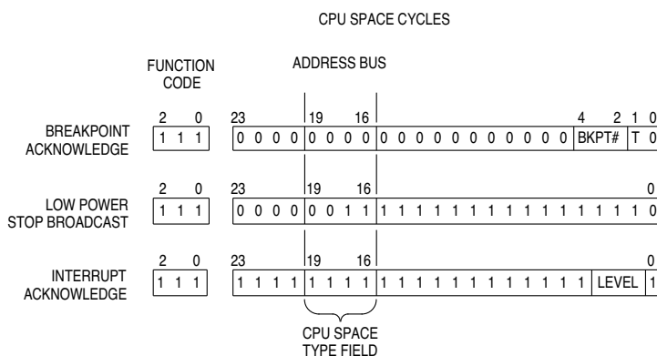
Figure 5-12 CPU Space Address Encoding
