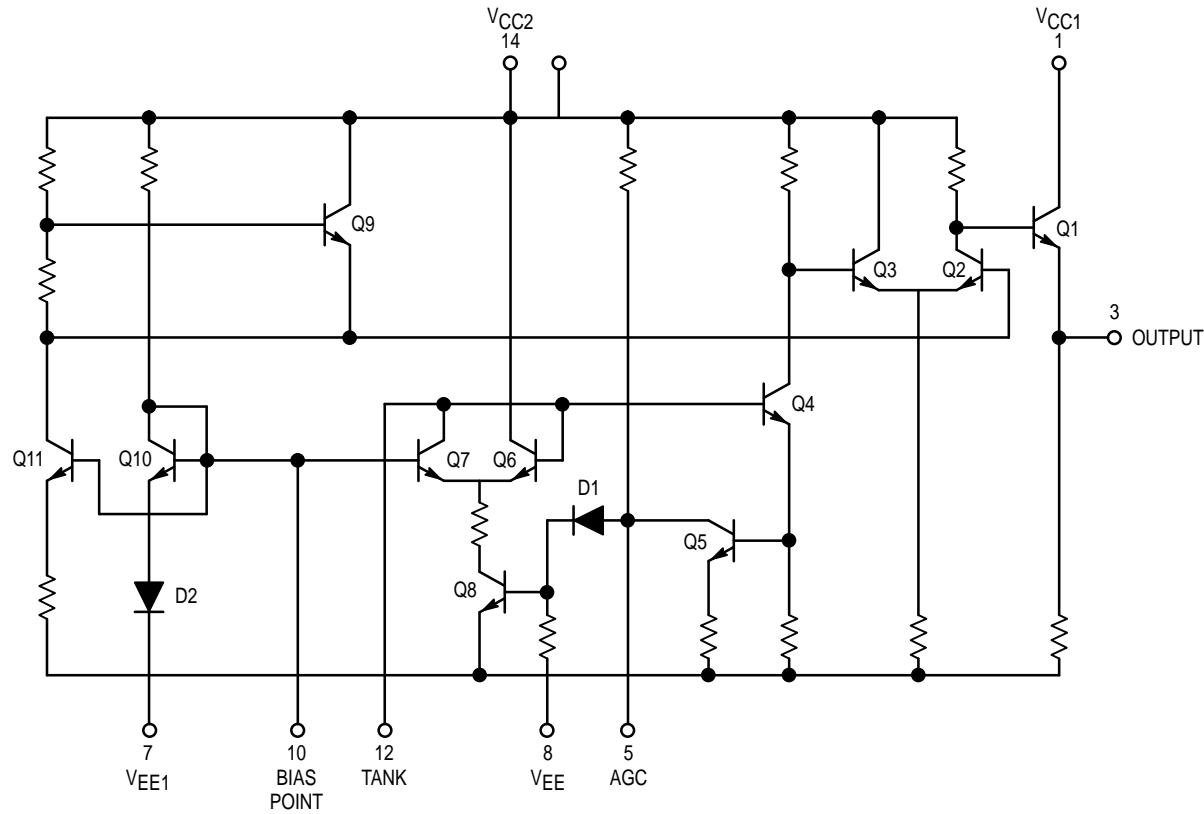
Figure 1. Circuit Schematic
