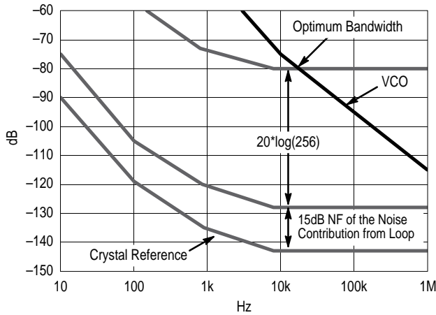
Figure 6. Graphical Analysis of Optimum Bandwidth
