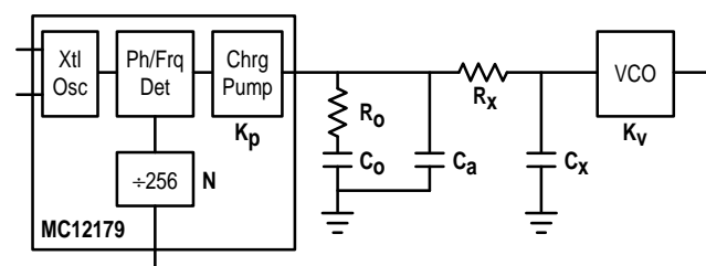
Figure 5. Loop Filter
