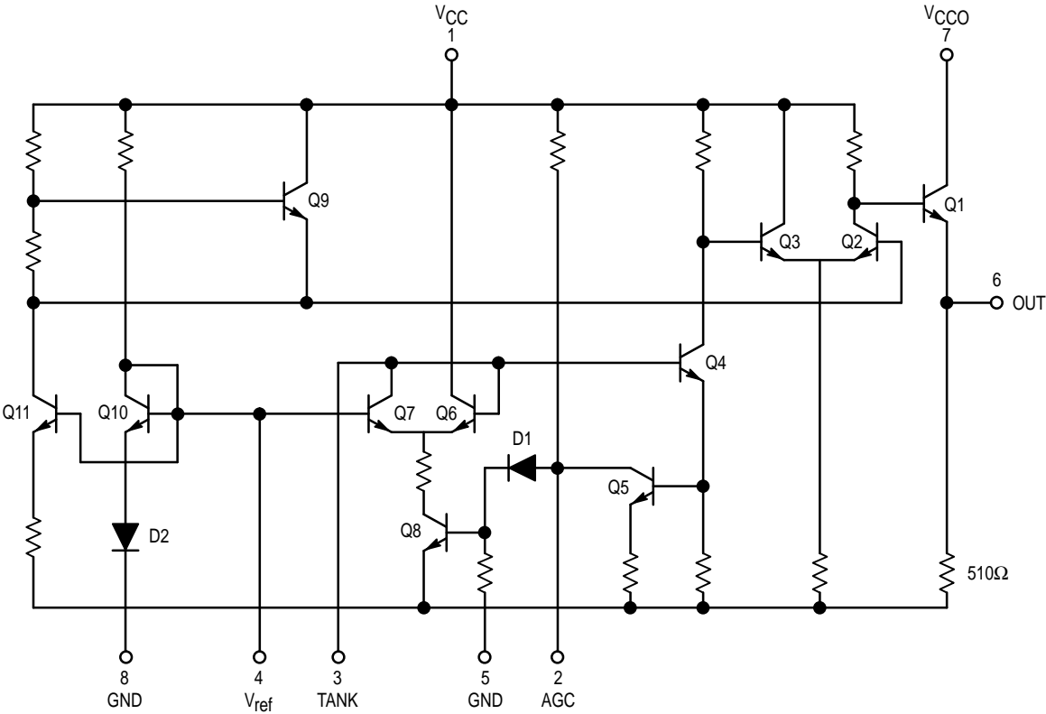
Figure 1. Circuit Schematic
